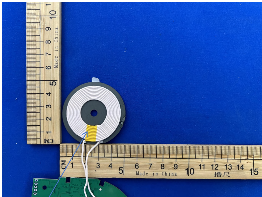
Wireless Charger antenna
