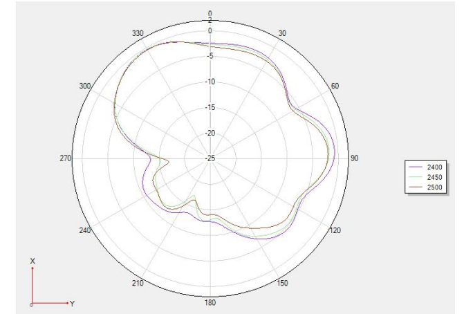
Theta 90 2Dgraph
