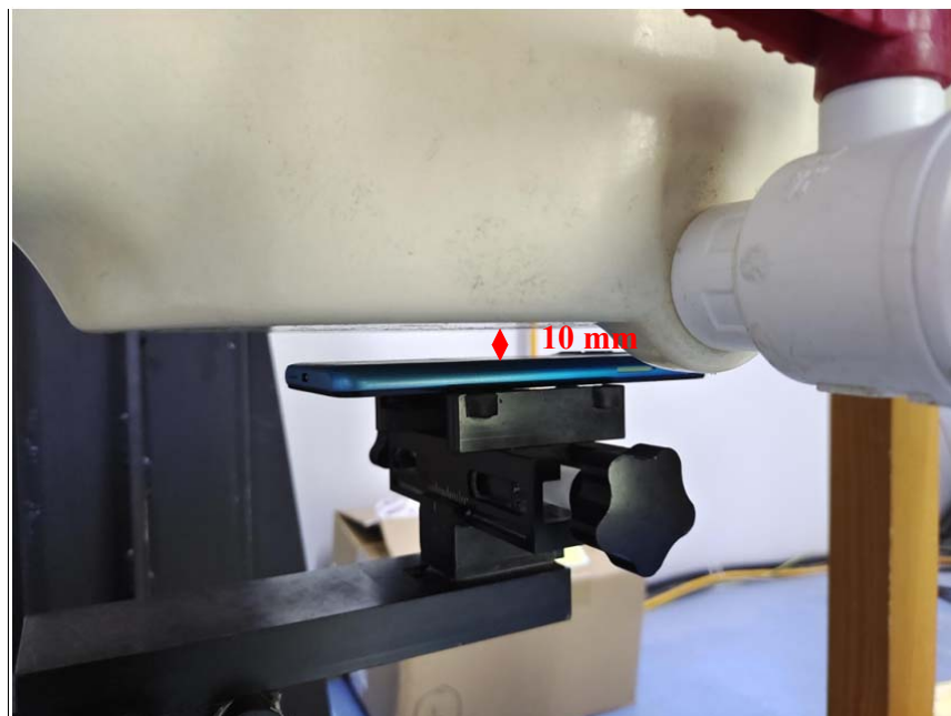
Body (Worn) Back Setup Photo (10mm)
