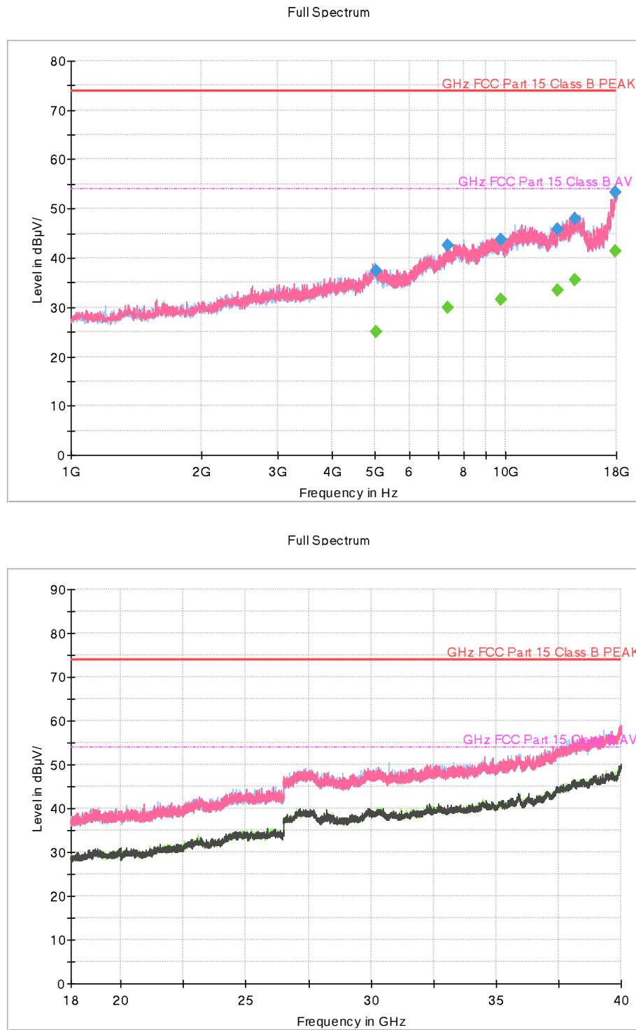
Figure 4: LTE B5+5G NR n5 Middle ch Idle
