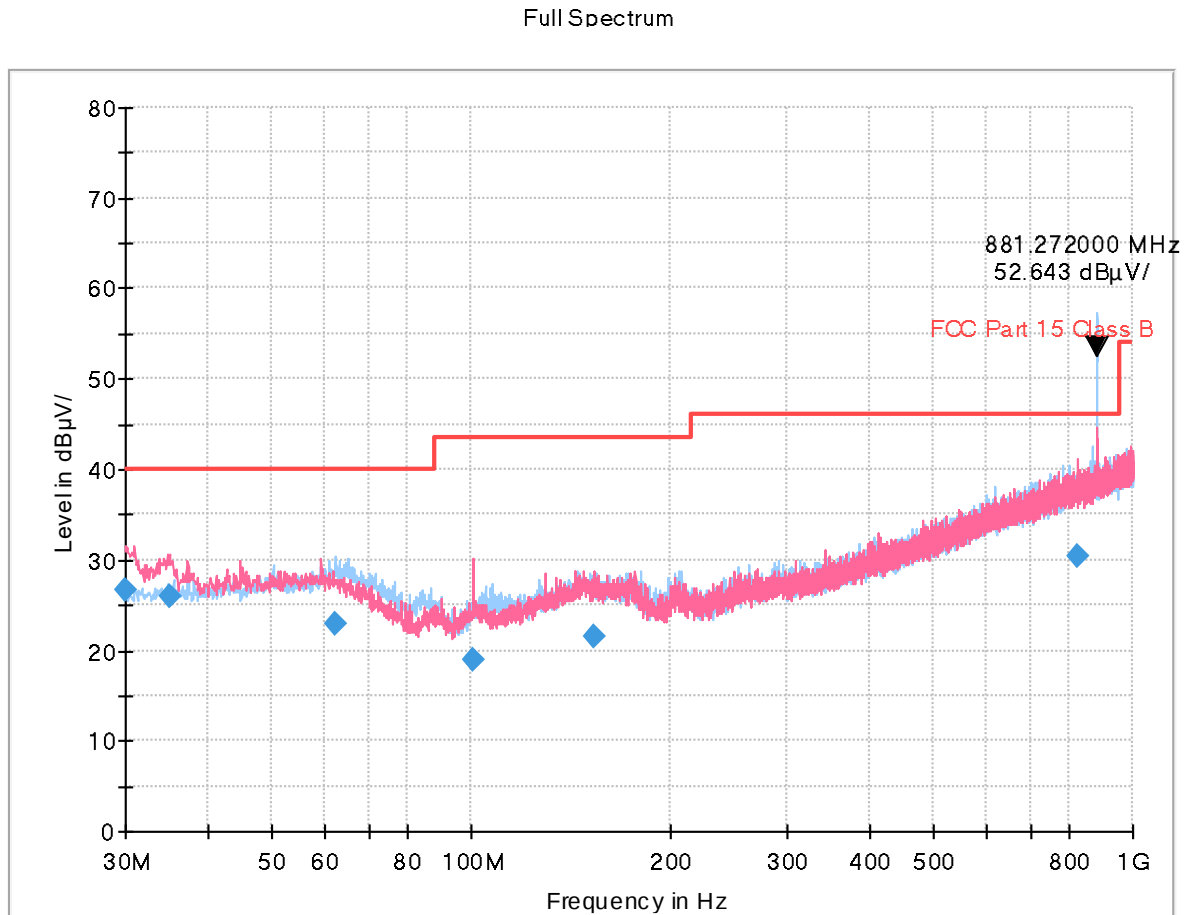
Figure 1: LTE B5+5G NR n5 Middle ch Idle
