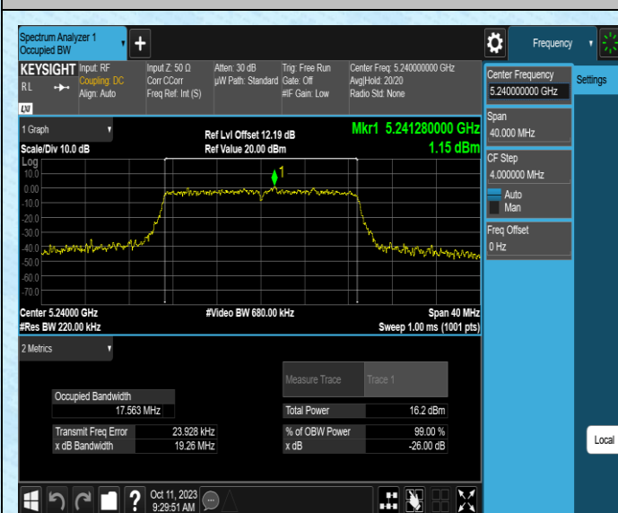
11AC20SISO-Ant1-5240
