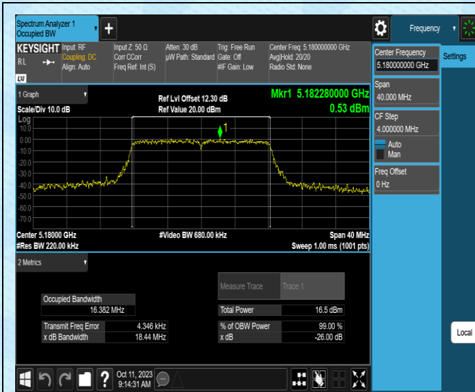
11A-Ant1-5180
