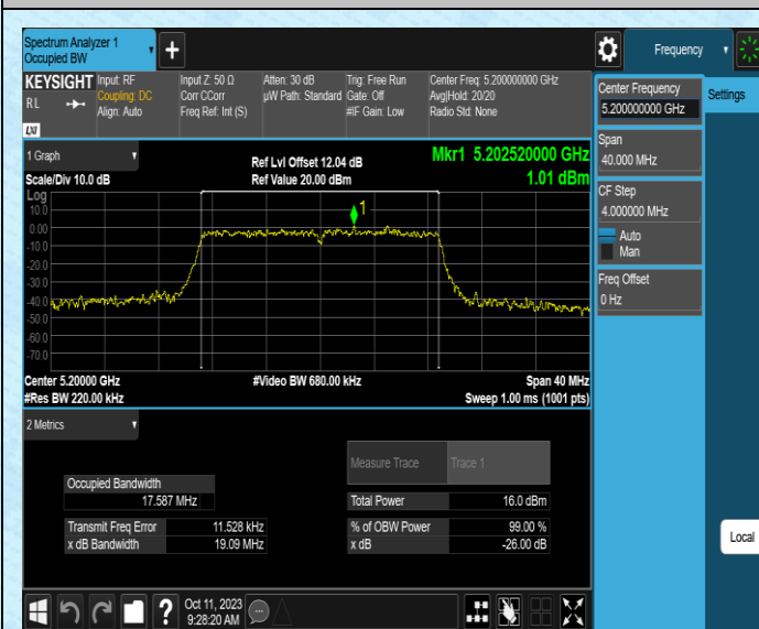
11AC20SISO-Ant1-5200
