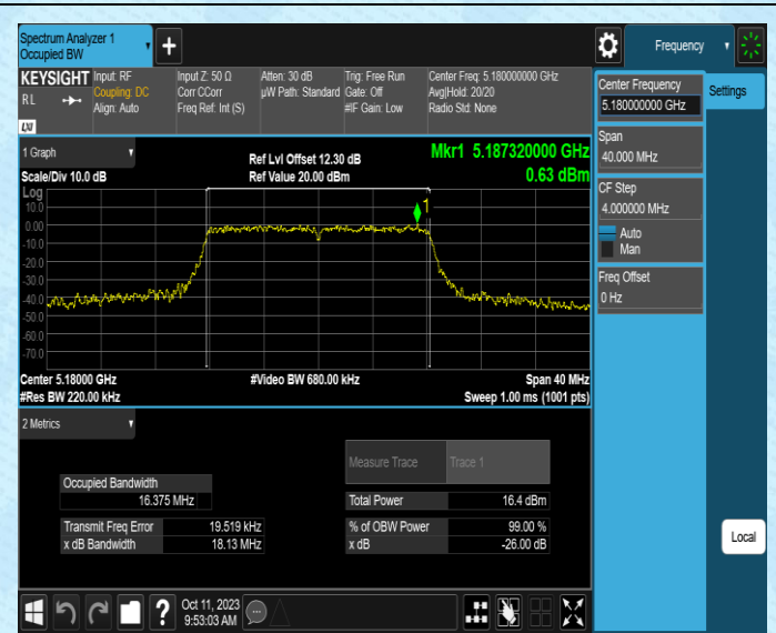
11A-Ant2-5180
