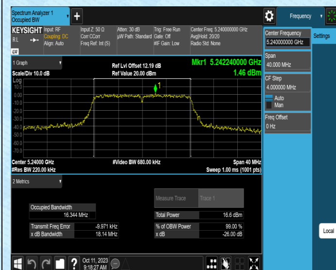
11A-Ant1-5240
