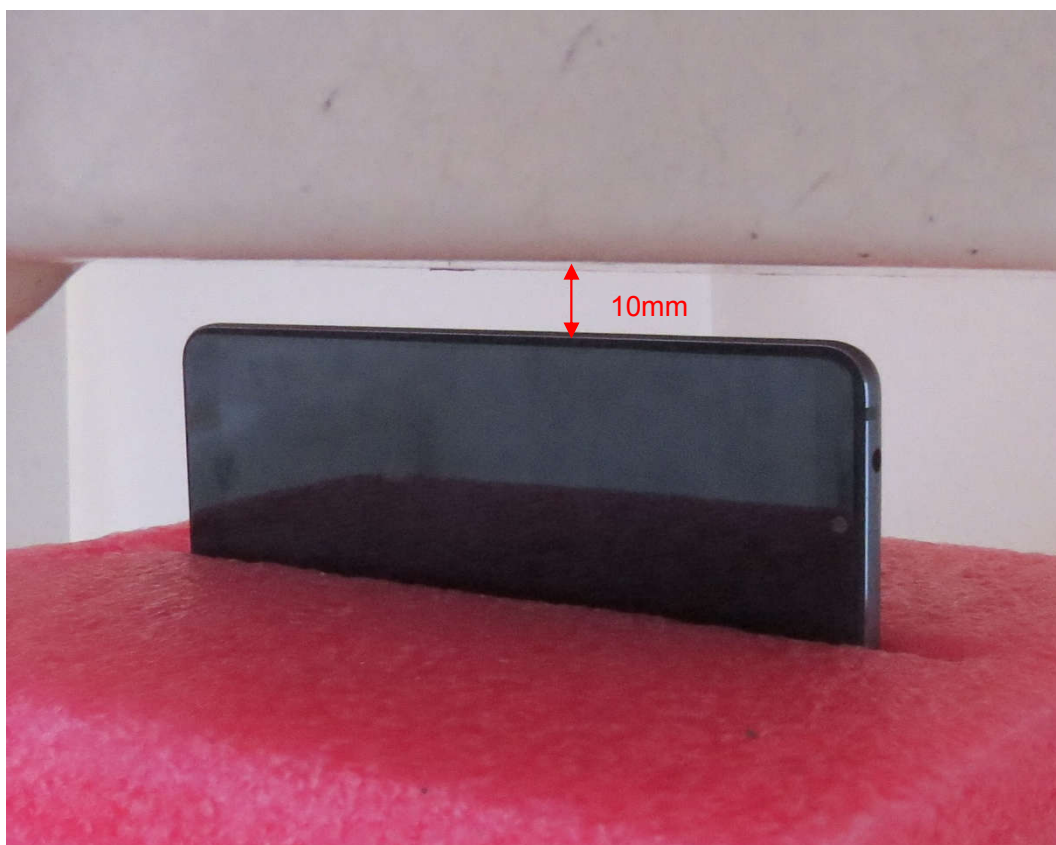
Picture 7: Left Side, the distance from handset to the bottom of the Phantom is 10mm
