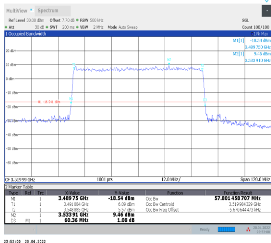
1-N78-3450-3550--30-60-H-9-CP-256QAM-Outer_Fu II-162@0-Ant0-57.801-60.360-≤60-PASS
