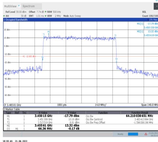
1-N78-3450-3550--30-70-L-1-DFT-QPSK-Outer_Full- 180@0-Ant0-64.21-66.360-≤70-PASS
