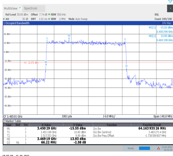
1-N78-3450-3550--30-70-L-2-DFT-PI2BPSK-Outer_F ull-180@0-Ant0-64.164-66.220-≤70-PASS
