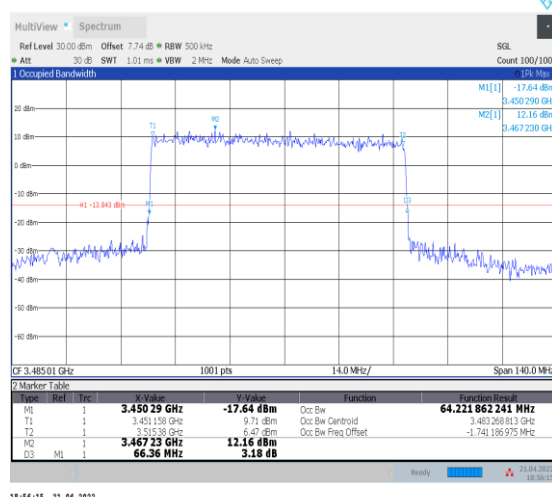
1-N78-3450-3550--30-70-L-3-DFT-16QAM-Outer_Fu ll-180@0-Ant0-64.222-66.360-≤70-PASS
