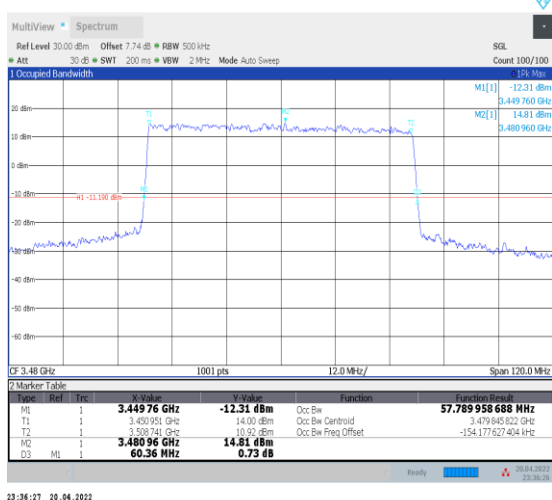
1-N78-3450-3550--30-60-L-1-DFT-QPSK-Outer_Full- 162@0-Ant0-57.79-60.360-≤60-PASS
