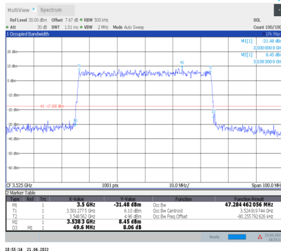
1-N78-3450-3550--30-50-H-9-CP-256QAM-Outer_F ull-133@0-Ant0-47.284-49.600-≤50-PASS
