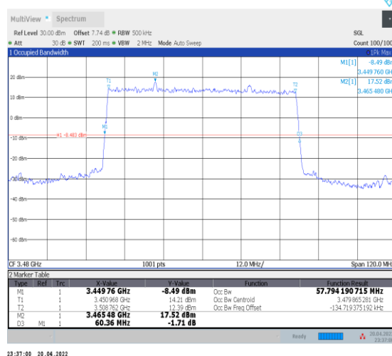
1-N78-3450-3550--30-60-L-2-DFT-PI2BPSK-Outer_ Full-162@0-Ant0-57.794-60.360-≤60-PASS
