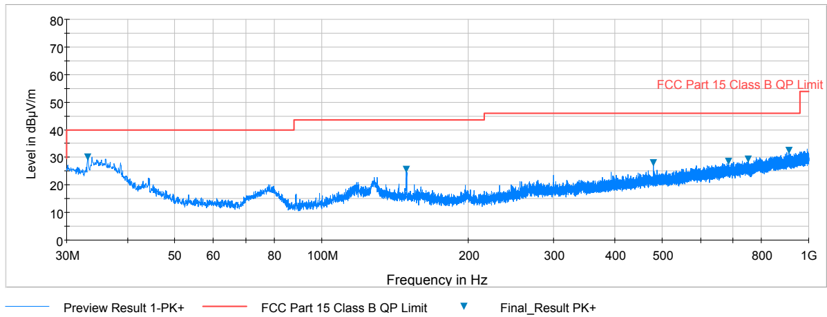
Plot 7-20. Radiated Spurious Plot below 1GHz (Pol. V)
