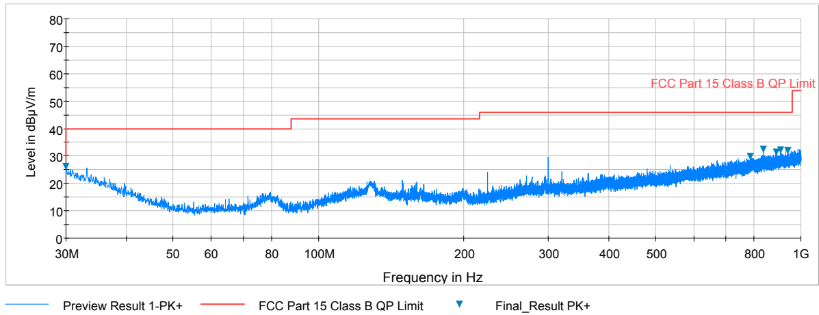
Plot 7-19. Radiated Spurious Plot below 1GHz (Pol. H)
