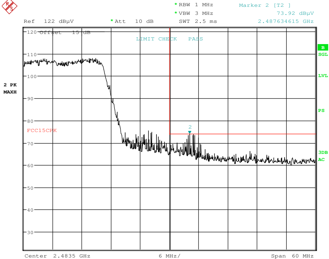
Plot 7-16. Radiated Restricted Upper Band Edge Measurement (Peak)
