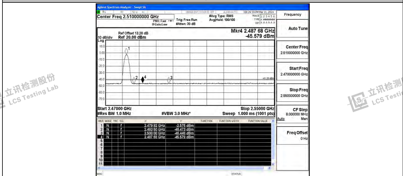
2DH5_Ant_High_2480_Peak
