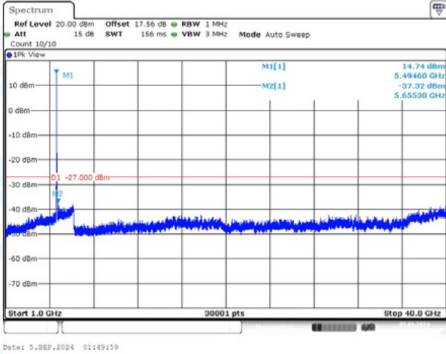
11AC20-CDD-Ant1-5500-1000~40000-PASS
