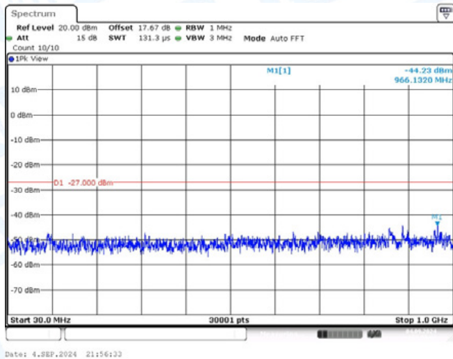
11N40-CDD-Ant2-5550-30~1000-PASS
