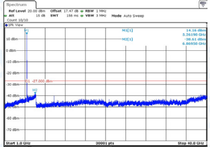
11N20-CDD-Ant1-5260-1000~40000-PASS
