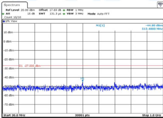
11N20-CDD-Ant2-5745-30~1000-PASS
