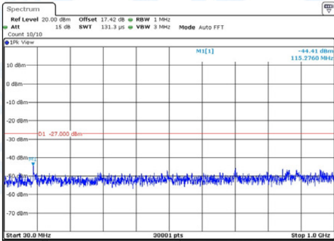
11N20-CDD-Ant2-5260-30~1000-PASS
