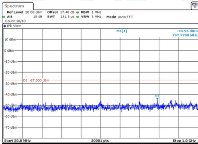
11N40-CDD-Ant2-5190-30~1000-PASS
