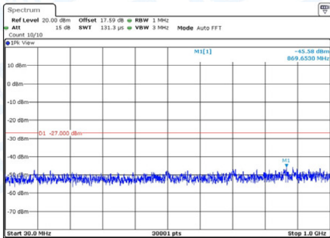
11N20-CDD-Ant2-5500-30~1000-PASS
