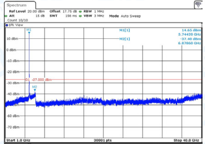
11N20-CDD-Ant1-5745-1000~40000-PASS
