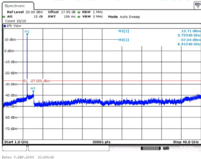
11AC20-CDD-Ant1-5720-1000~40000-PASS
