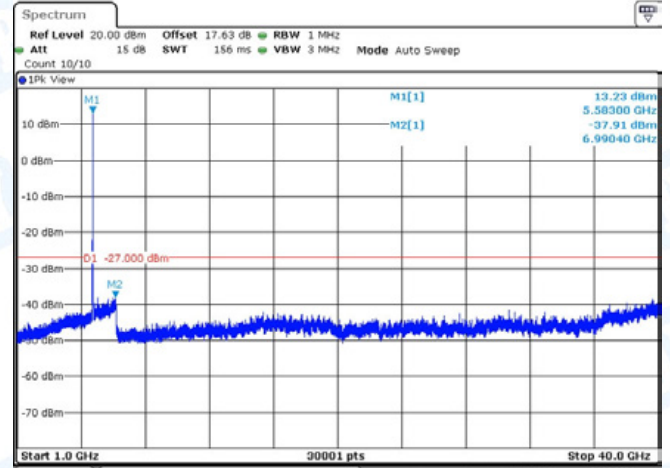
11N20-CDD-Ant2-5580-1000~40000-PASS
