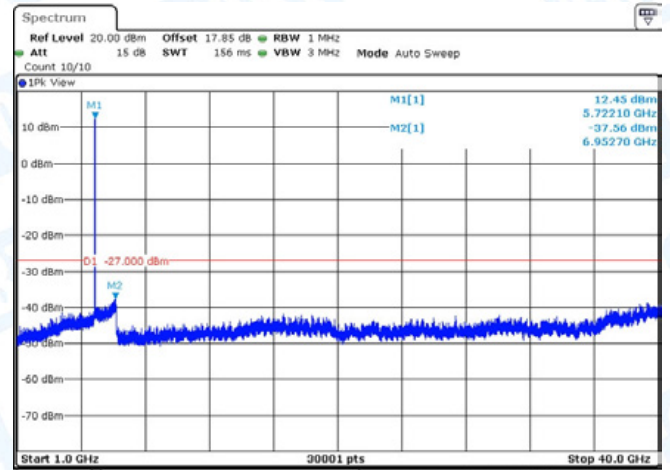
11N20-CDD-Ant1-5720-1000~40000-PASS
