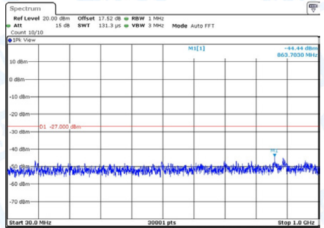
11AC20-CDD-Ant1-5280-30~1000-PASS
