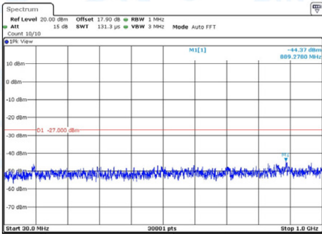
11N20-CDD-Ant2-5580-30~1000-PASS
