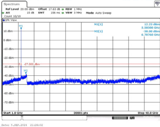
11AC20-CDD-Ant2-5580-1000~40000-PASS
