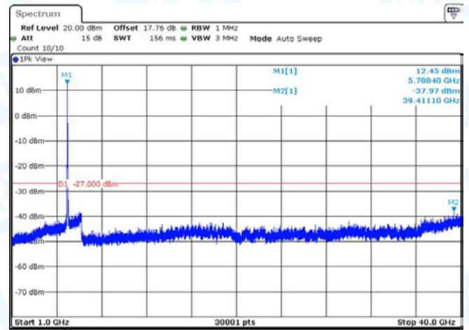
11N40-CDD-Ant1-5795-1000~40000-PASS
