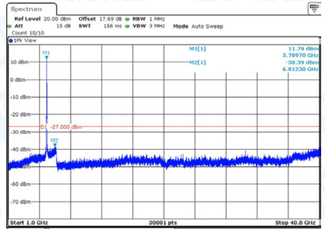
11N40-CDD-Ant2-5755-1000~40000-PASS
