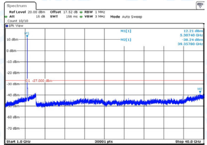
11N40-CDD-Ant1-5310-1000~40000-PASS
