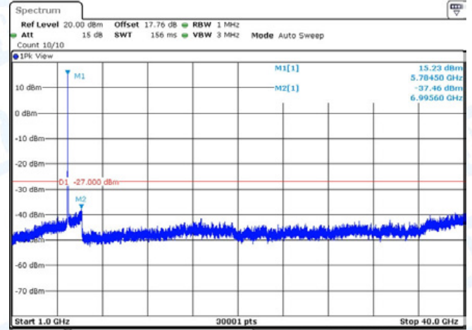
11N20-CDD-Ant2-5785-1000~40000-PASS
