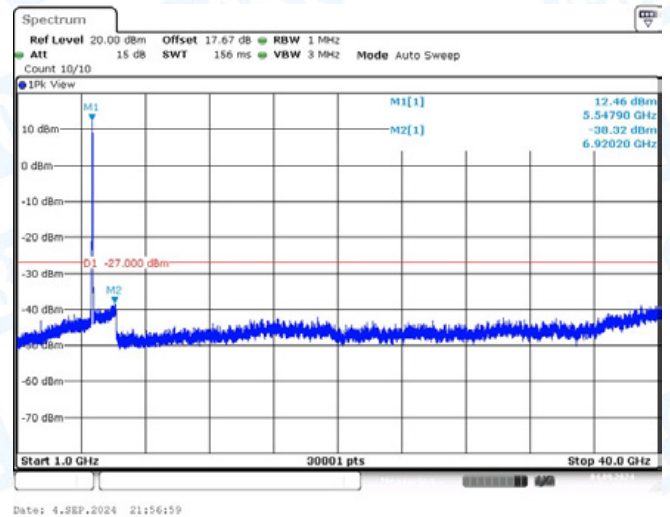
11N40-CDD-Ant2-5550-1000~40000-PASS
