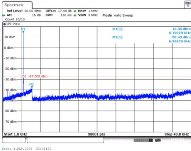
11AC20-CDD-Ant2-5200-1000~40000-PASS
