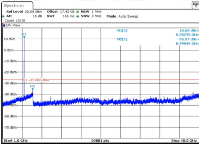
11AC20-CDD-Ant2-5260-1000~40000-PASS
