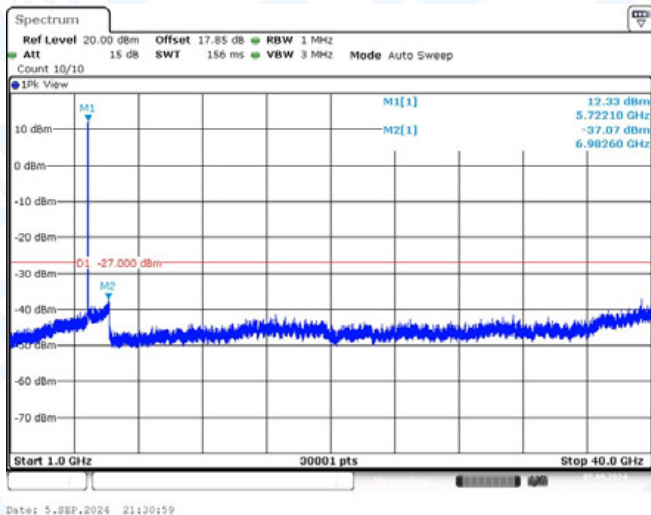
11AC20-CDD-Ant2-5720-1000~40000-PASS
