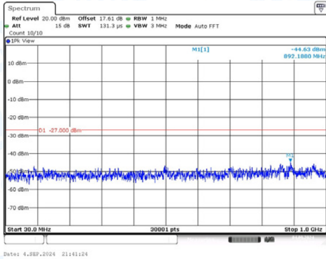
11N40-CDD-Ant2-5510-30~1000-PASS
