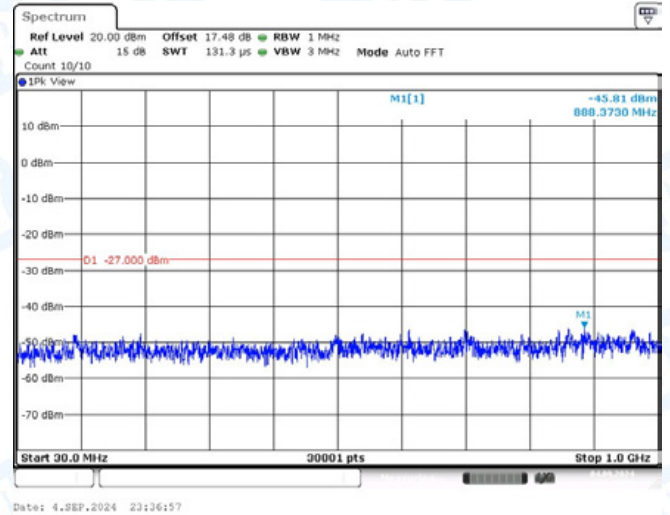
11AC20-CDD-Ant1-5240-30~1000-PASS
