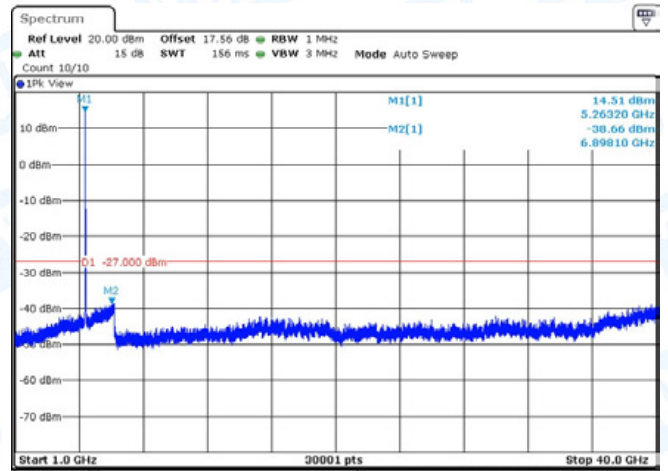
11N20-CDD-Ant1-5260-1000~40000-PASS
