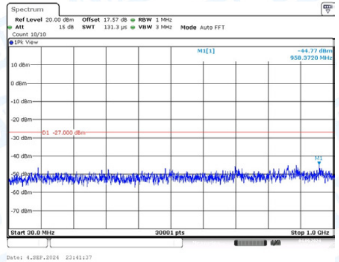
11AC20-CDD-Ant2-5240-30~1000-PASS
