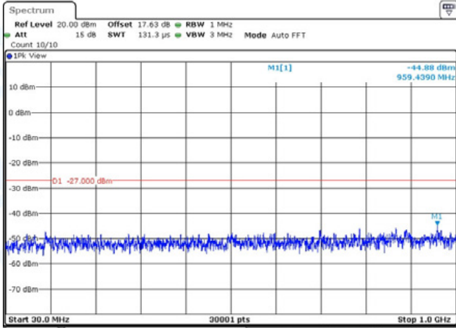
11N20-CDD-Ant2-5580-30~1000-PASS
