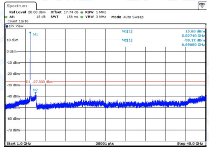
11N20-CDD-Ant2-5785-1000~40000-PASS
