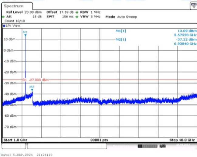
11AC20-CDD-Ant1-5580-1000~40000-PASS
