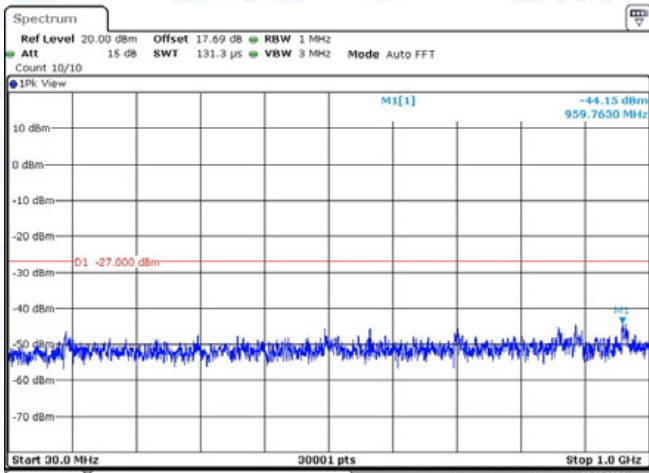
11N40-CDD-Ant2-5755-30~1000-PASS
