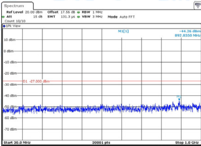
11N20-CDD-Ant1-5260-30~1000-PASS
