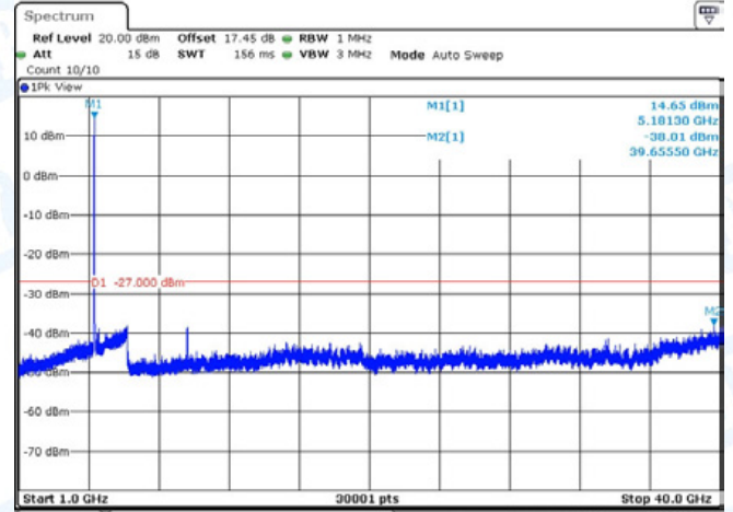
11AC20-CDD-Ant1-5180-1000~40000-PASS
