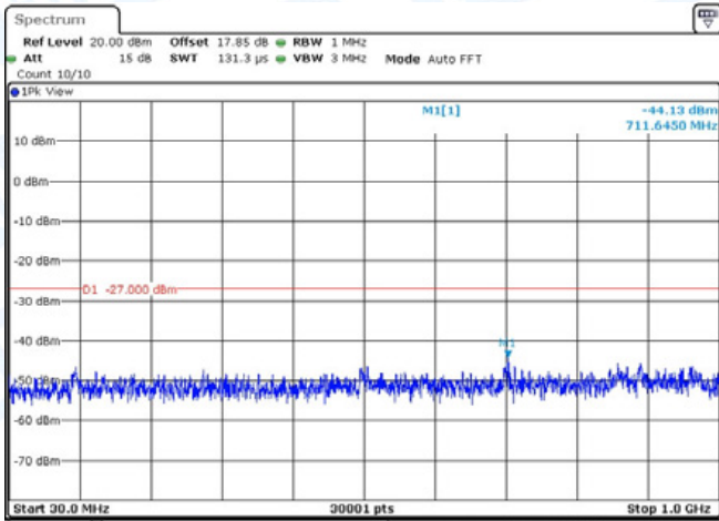
11N20-CDD-Ant1-5825-30~1000-PASS
