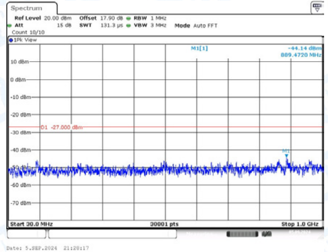
11AC20-CDD-Ant1-5720-30~1000-PASS
