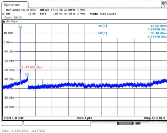
11AC20-CDD-Ant1-5240-1000~40000-PASS
