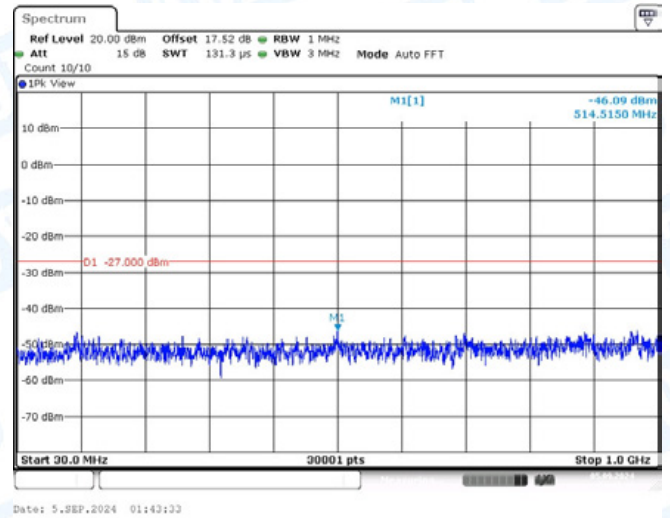
11AC20-CDD-Ant2-5320-30~1000-PASS
