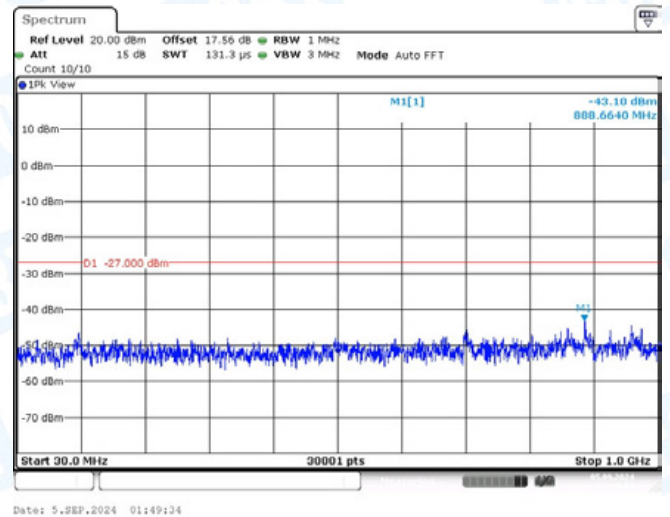
11AC20-CDD-Ant1-5500-30~1000-PASS
