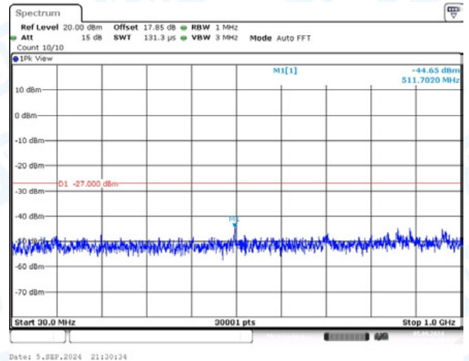
11AC20-CDD-Ant2-5720-30~1000-PASS
