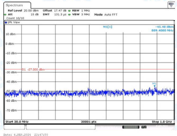
11AC20-CDD-Ant1-5260-30~1000-PASS
