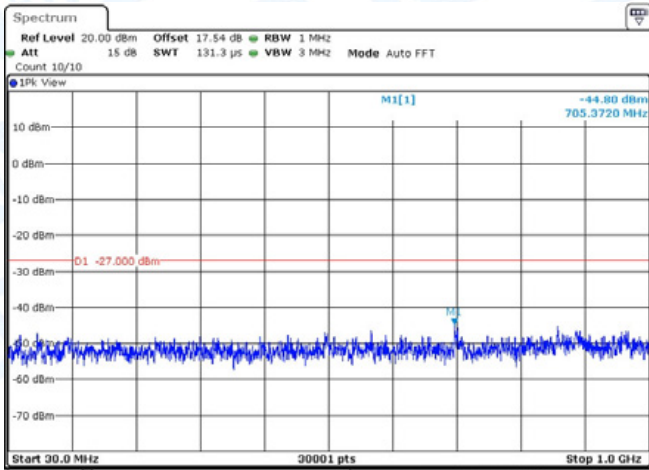
11N40-CDD-Ant2-5310-30~1000-PASS
