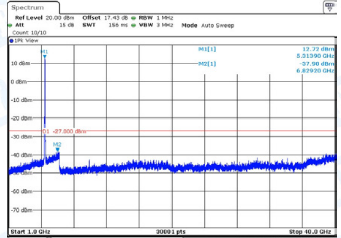
11N40-CDD-Ant1-5310-1000~40000-PASS
