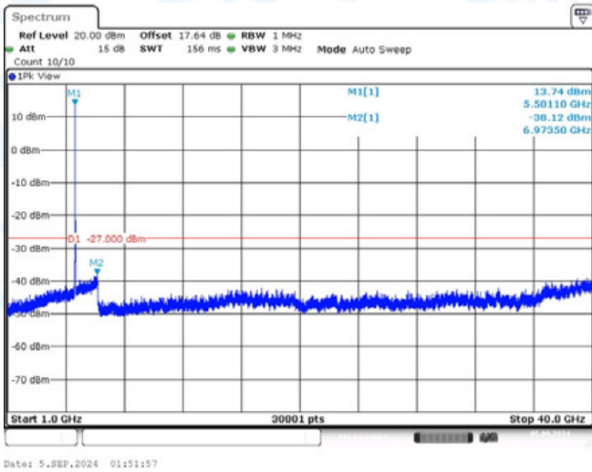
11AC20-CDD-Ant2-5500-1000~40000-PASS
