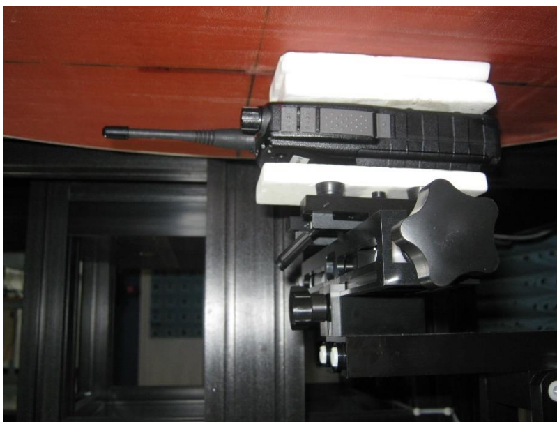
Figure 42 Front of Face PTT - 1880 mAh battery 25mm separation distance
