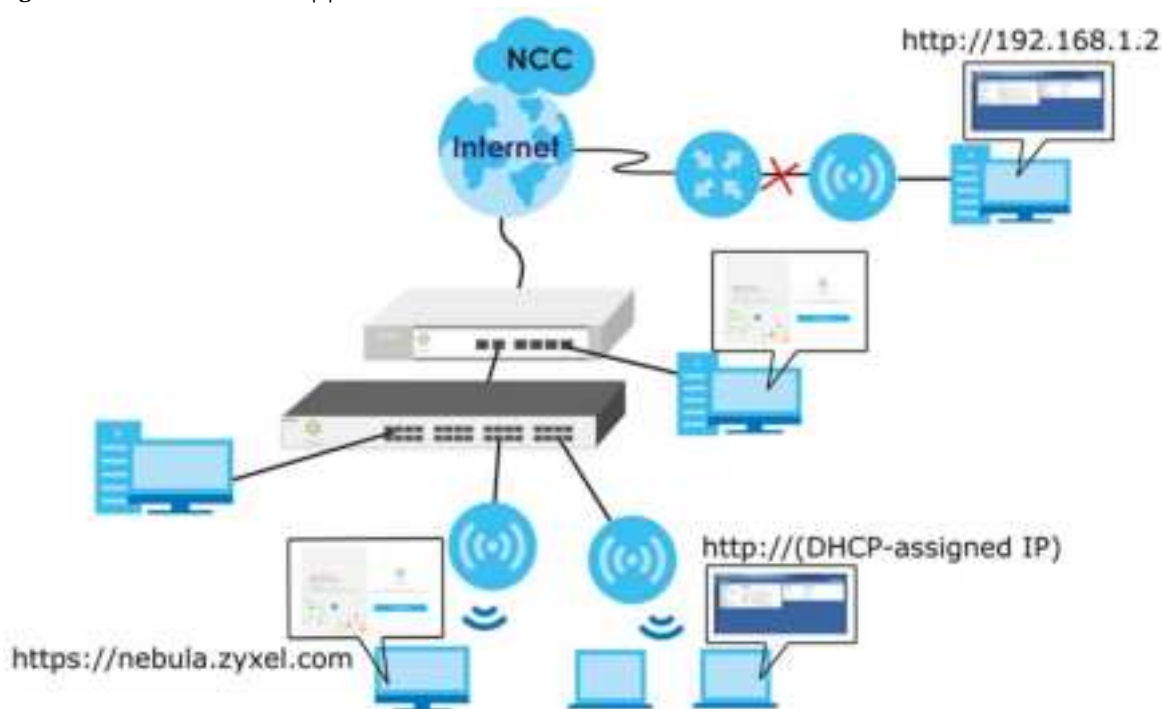
Figure 160 Cloud Mode Application
