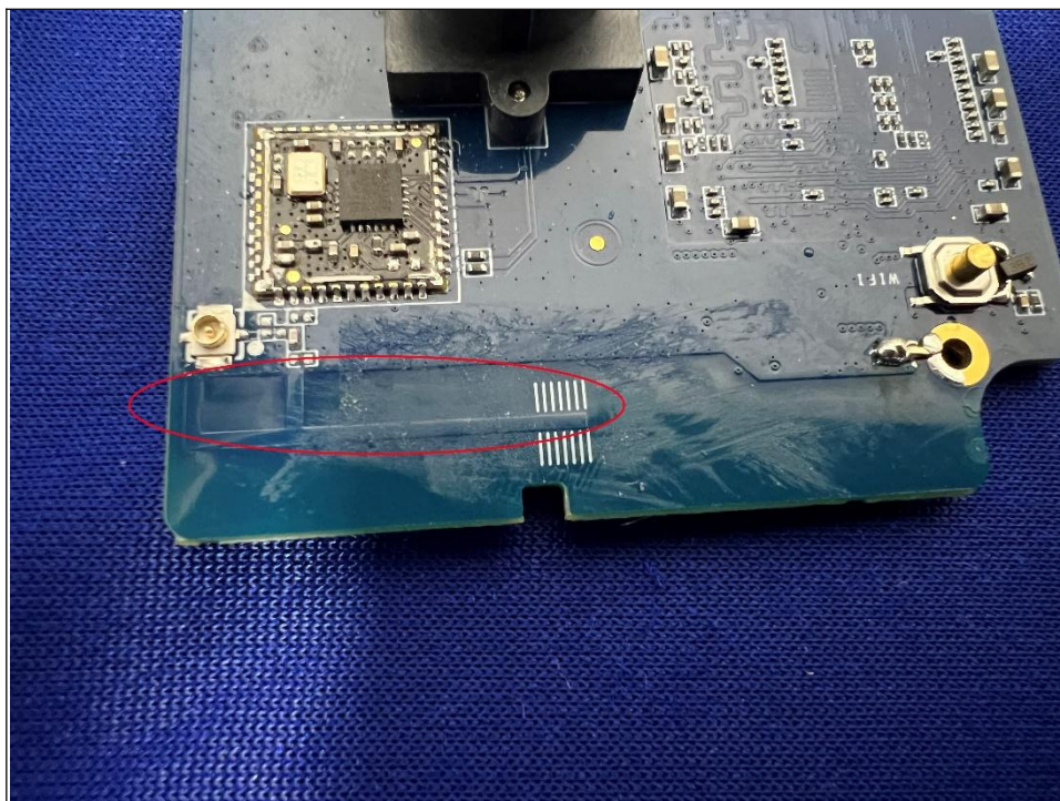
WIFI ANTENNA
