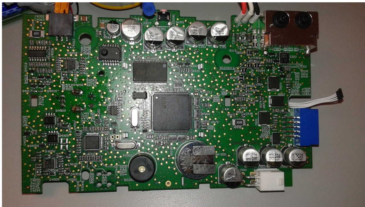
Back of Flow Generator Mother Board
