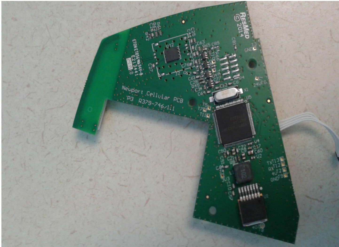
CPU side of CAM Board
