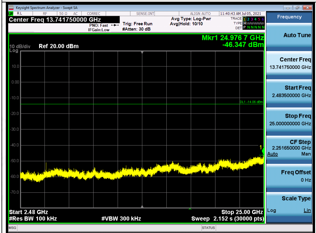
Test_Graph_CCK_ANT1_2437_1Mbps_Higher Band Emissions
