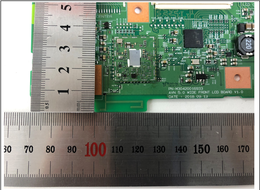
<WiFi Antenna>
