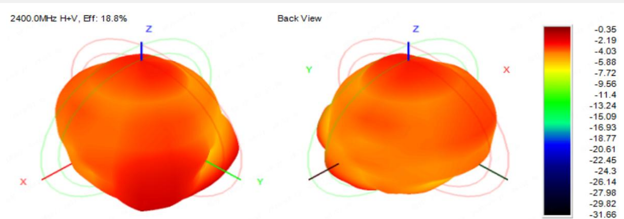
3D Pattern for 2400MHz
