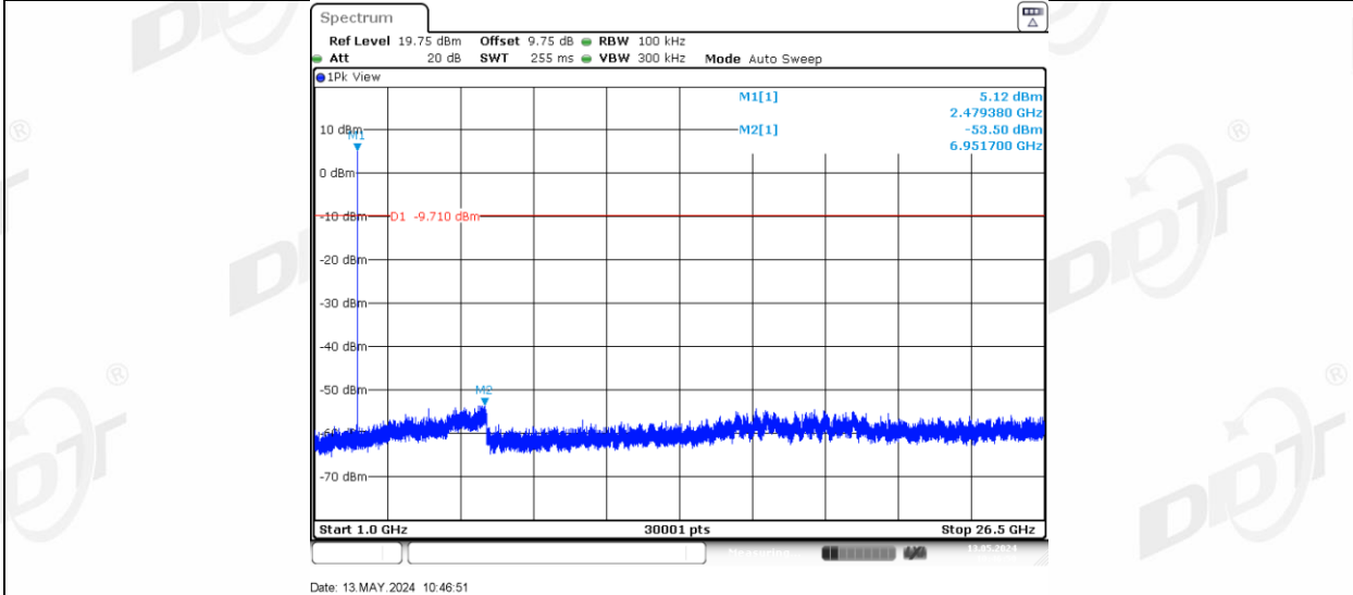
3DH5_Right side_2480_0~Reference
