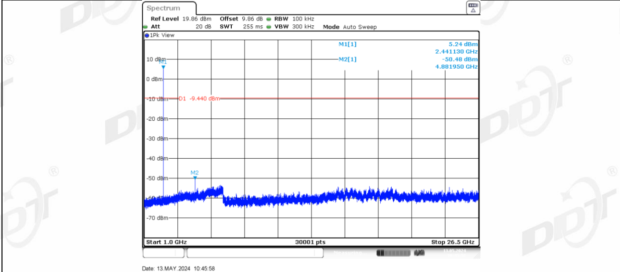
3DH5_Right side_2441_0~Reference
