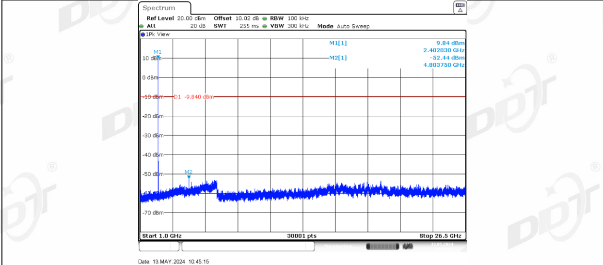
3DH5_Right side_2402_0~Reference
