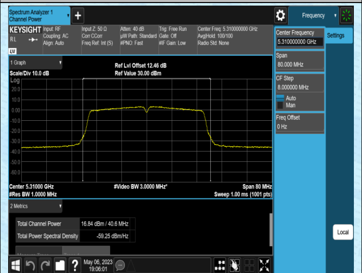
11AC40SISO-Ant2-5310
