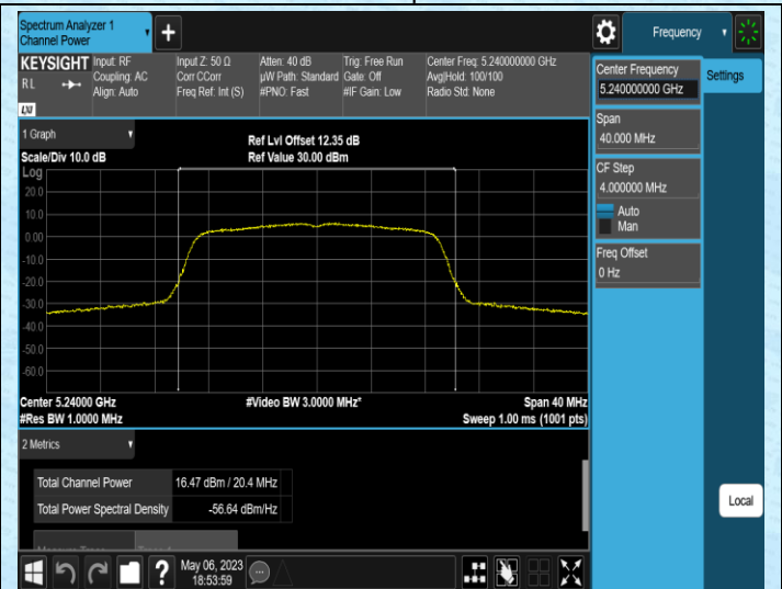
11AC20SISO-Ant2-5240
