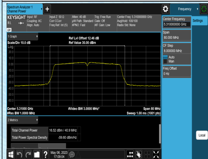
11AC40SISO-Ant1-5310
