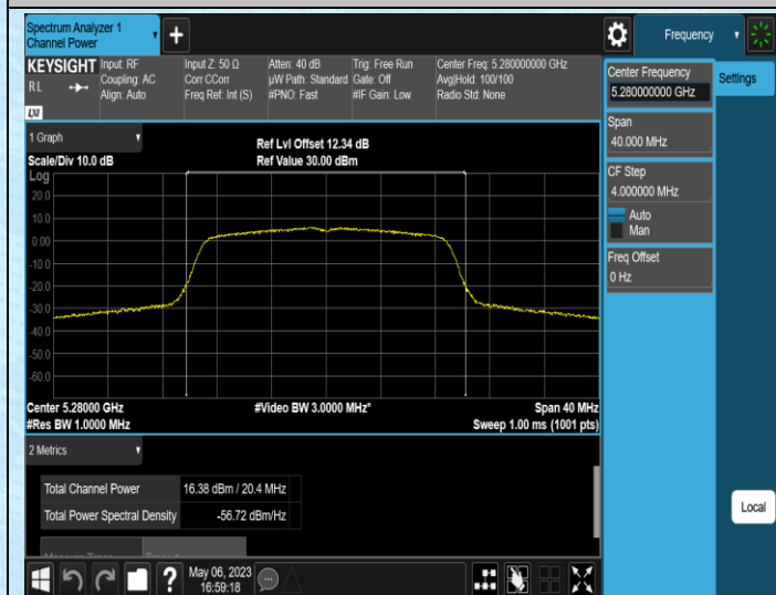
11AC20SISO-Ant1-5280
