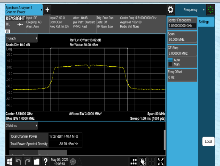
11AC40SISO-Ant2-5510
