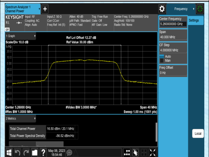
11AC20SISO-Ant2-5260
