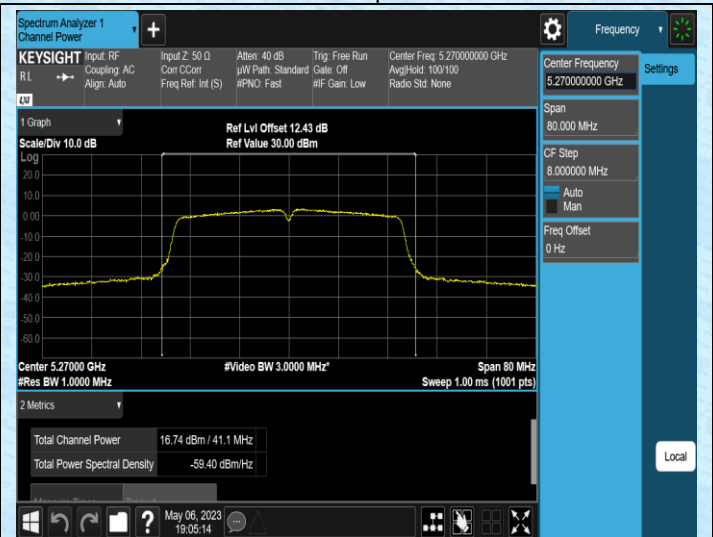
11AC40SISO-Ant2-5270
