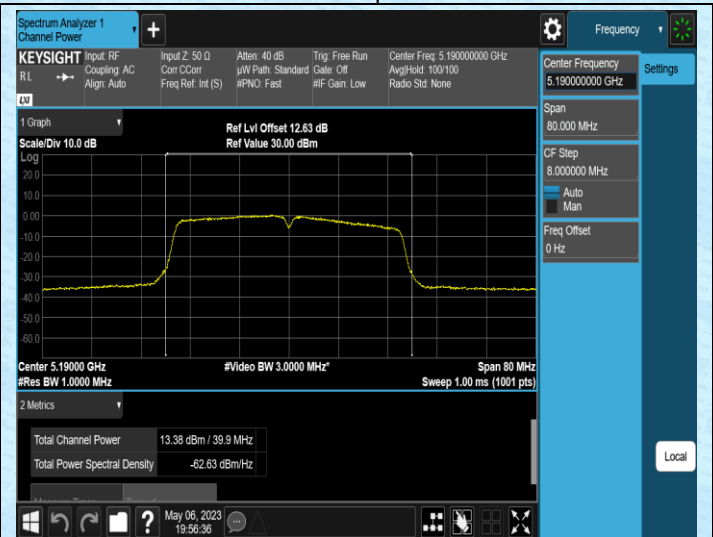
11N40MIMO-Ant2-5190
