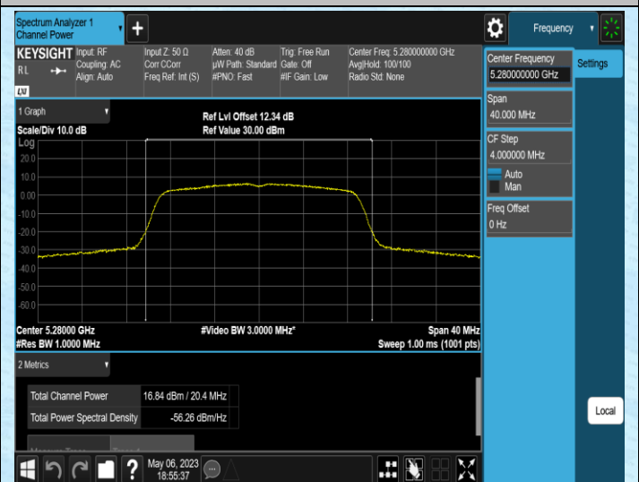
11AC20SISO-Ant2-5280
