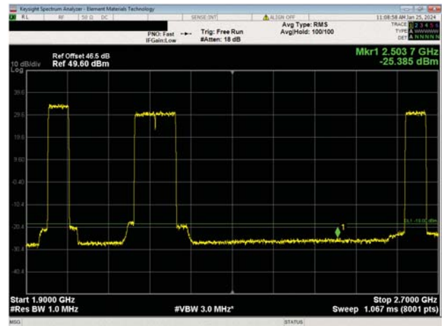
AWS Multicarrier Multiband Test Case 2 QPSK Modulation 1.9 GHz - 2.7 GHz
