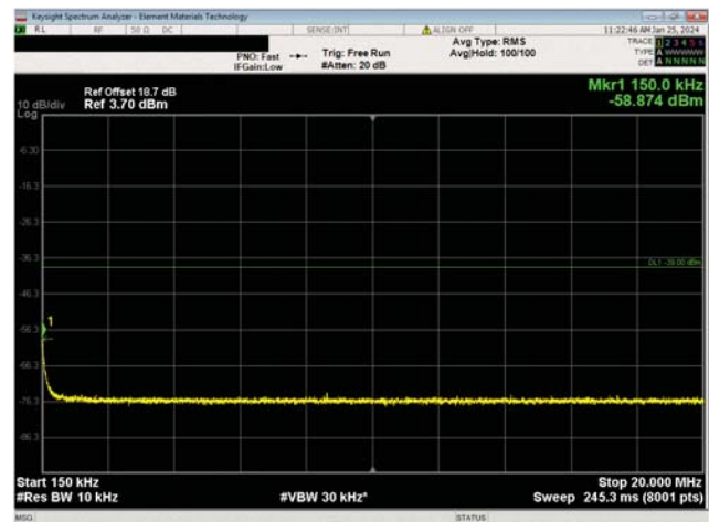
AWS Multicarrier Multiband Test Case 3 QPSK Modulation 150 kHz - 20 MHz
