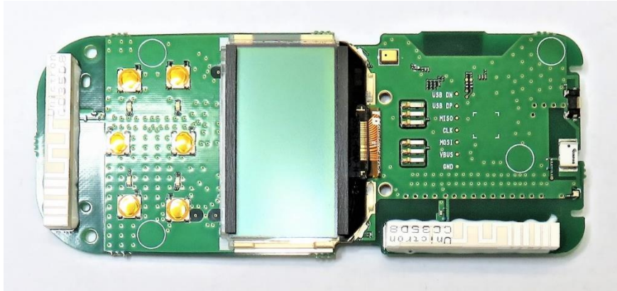
Front Board side-A view
