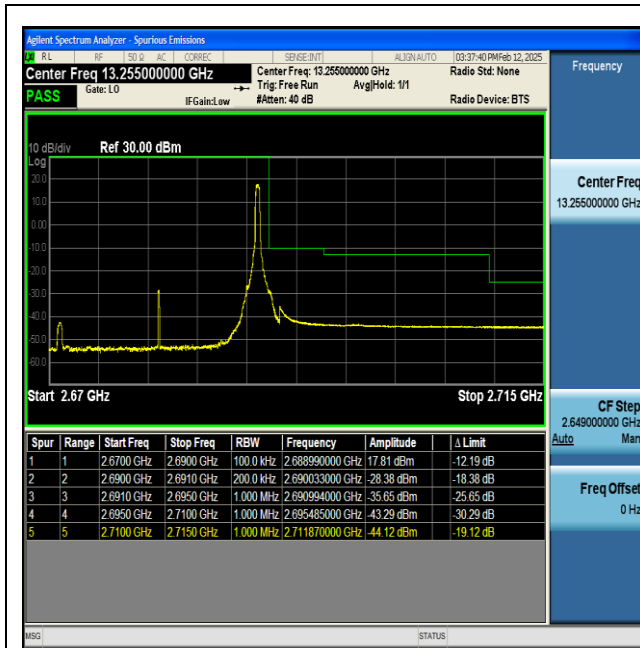
NTNV-n41-PC2-30-20-H-DFT-BPSK-Edge_1RB_Right-PASS
