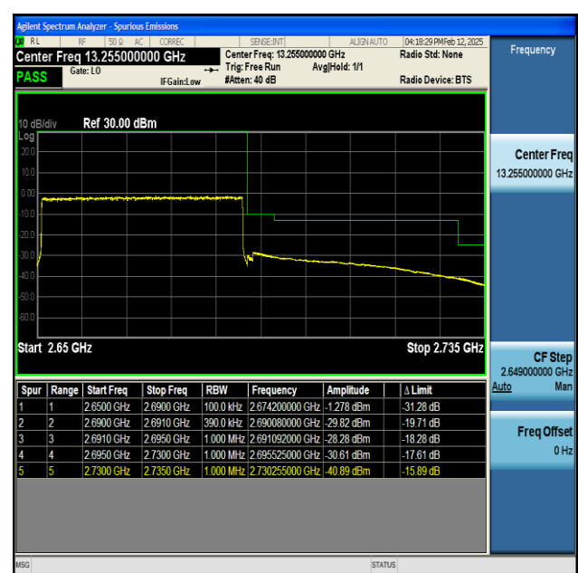
NTNV-n41-PC2-30-40-H-CP-QPSK-Outer_Full-PASS
