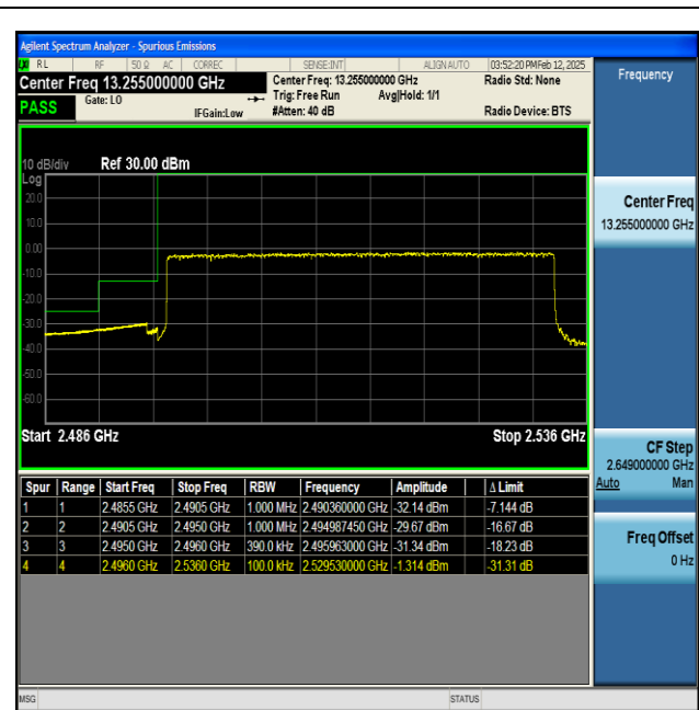
NTNV-n41-PC2-30-40-L-DFT-BPSK-Outer_Full-PASS
