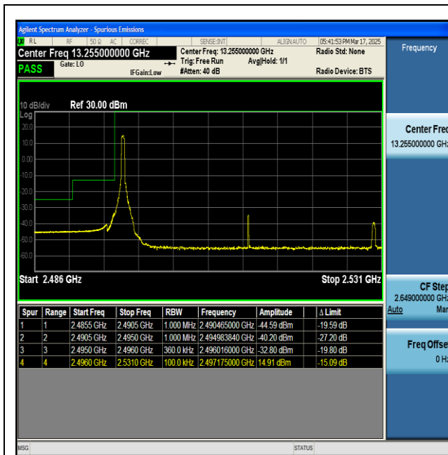
NTNV-n41-PC2-30-35-L-DFT-BPSK-Edge_1RB_Left-PASS
