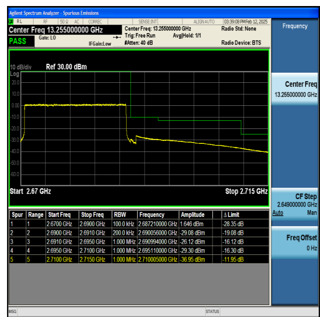
NTNV-n41-PC2-30-20-H-CP-QPSK-Outer_Full-PASS
