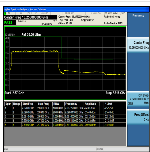
NTNV-n41-PC2-30-20-H-DFT-BPSK-Outer_Full-PASS
