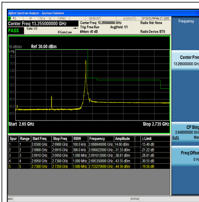
NTNV-n41-PC2-30-40-H-DFT-BPSK-Edge_1RB_Right-PASS
