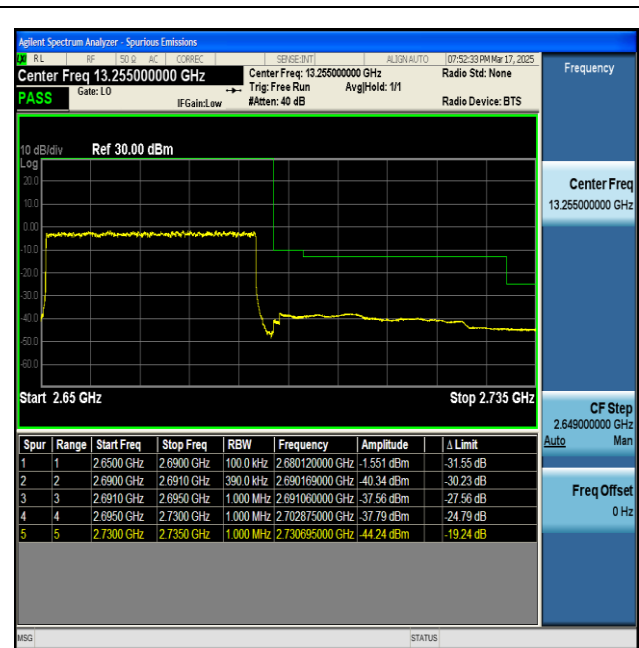
NTNV-n41-PC2-30-40-H-DFT-BPSK-Outer_Full-PASS
