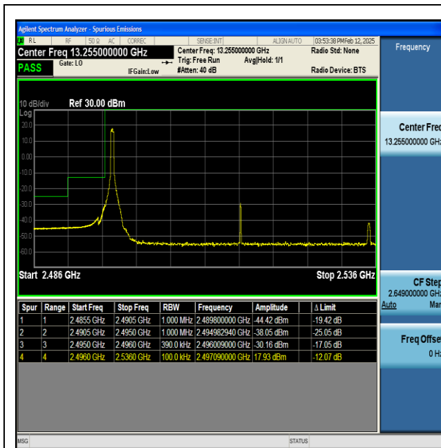
NTNV-n41-PC2-30-40-L-DFT-BPSK-Edge_1RB_Left-PASS
