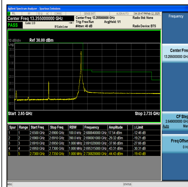
NTNV-n41-PC2-30-40-H-CP-QPSK-Edge_1RB_Right-PASS
