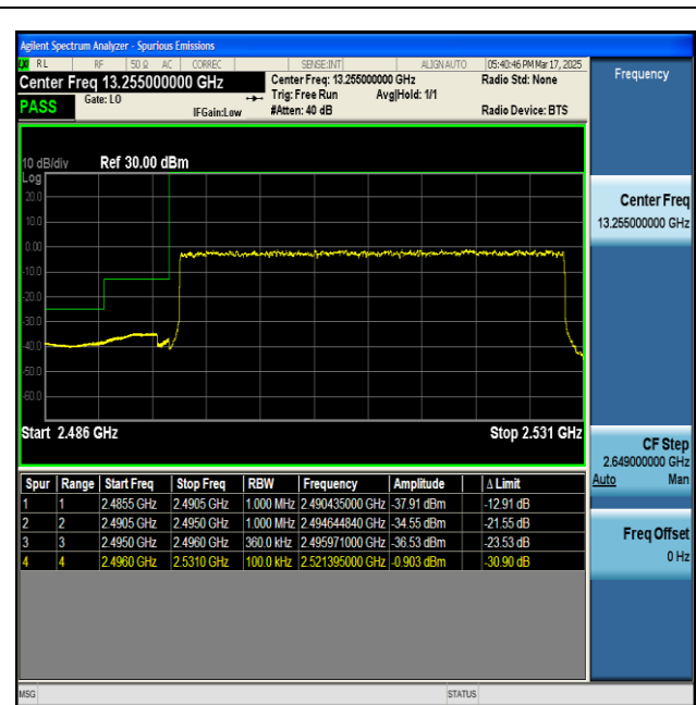
NTNV-n41-PC2-30-35-L-DFT-BPSK-Outer_Full-PASS
