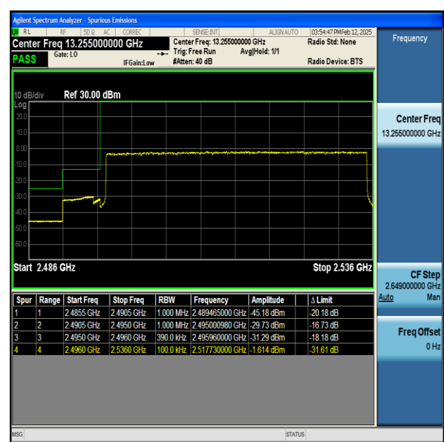
NTNV-n41-PC2-30-40-L-CP-QPSK-Outer_Full-PASS
