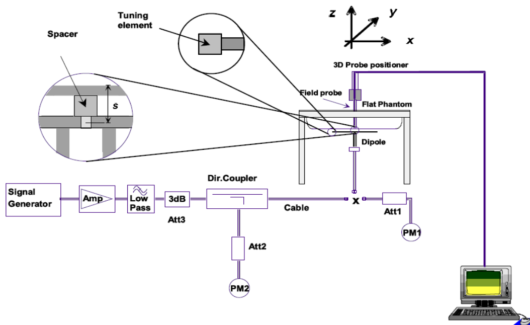
System Check Set-up
