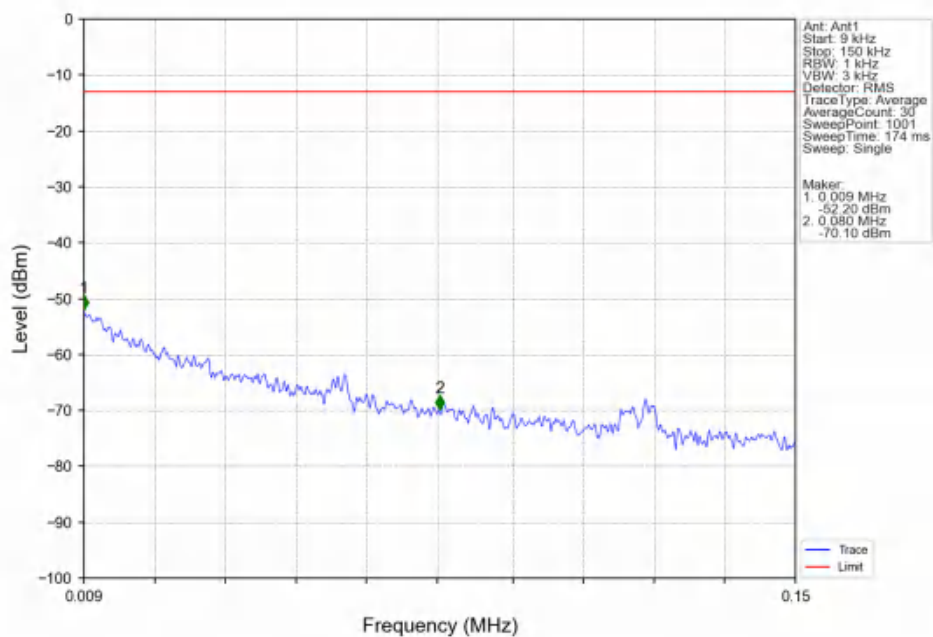
Band66 10MHz 16QAM HCH 1775MHz RB 1 0 NTNV
