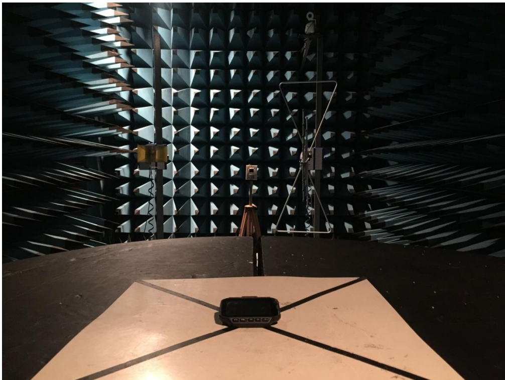
FCC Part15E Radiated Emission above 18-26.5GHz
