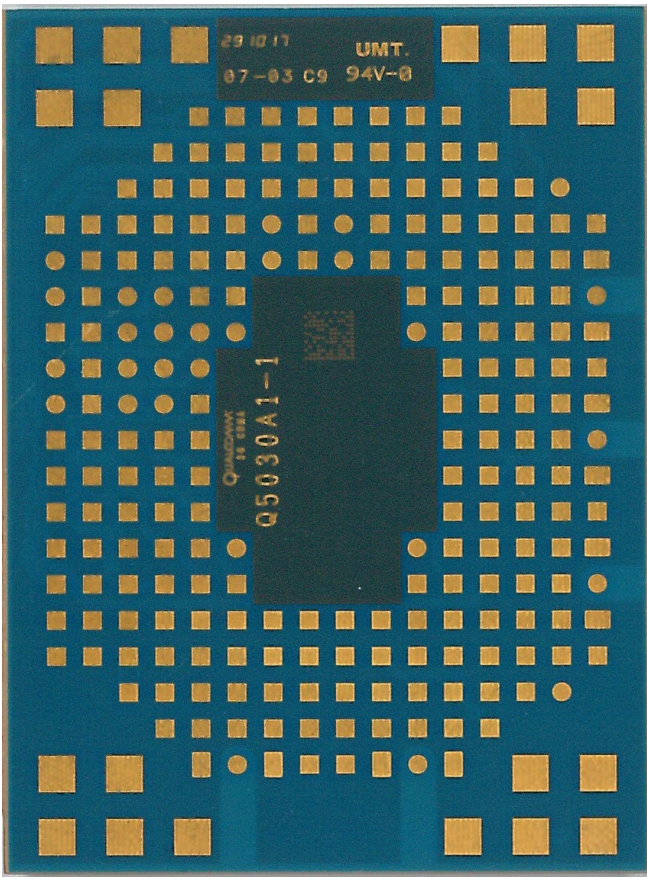
BOTTOM VIEW
