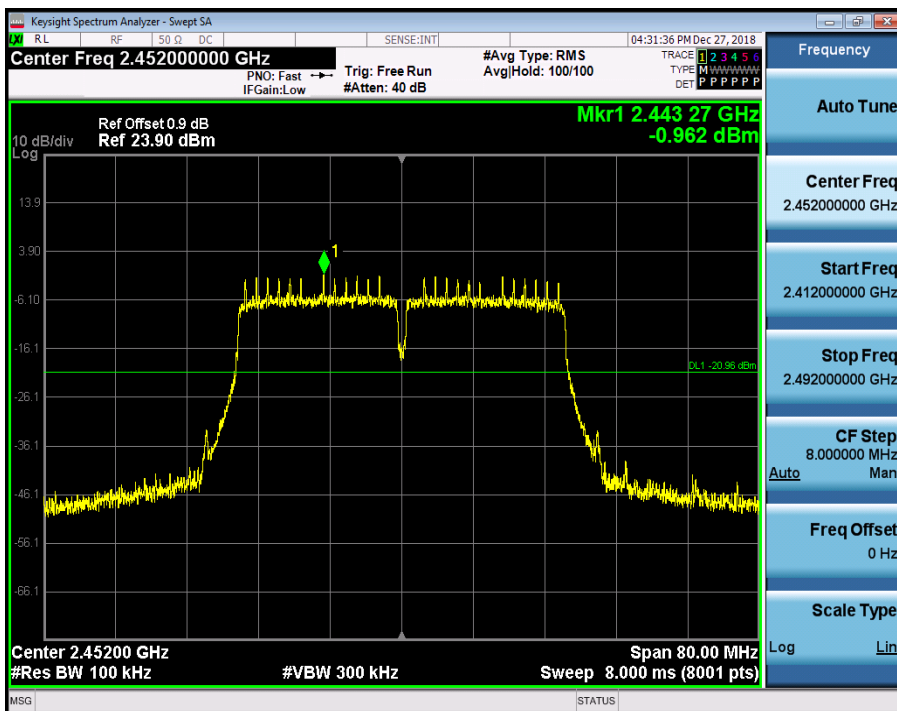
RF Conducted Spurious Emissions_11N40SISO_2452_Ant1
