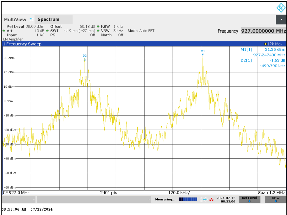
Figure 22 – ASK, 926.75 MHz / 927.25 MHz
