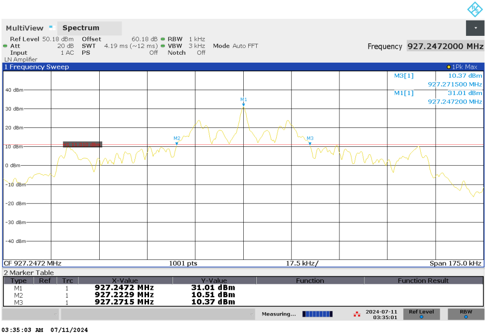
Figure 26 – ASK, 927.25 MHz
