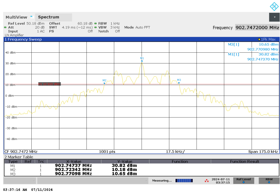
Figure 24 - ASK, 902.75 MHz
