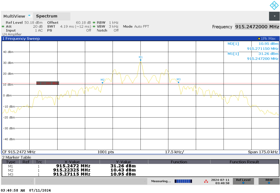
Figure 25 - ASK, 915.25 MHz
