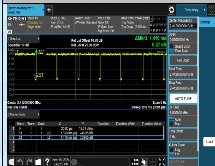
NTNV-11N20SISO-Ant1-2412
