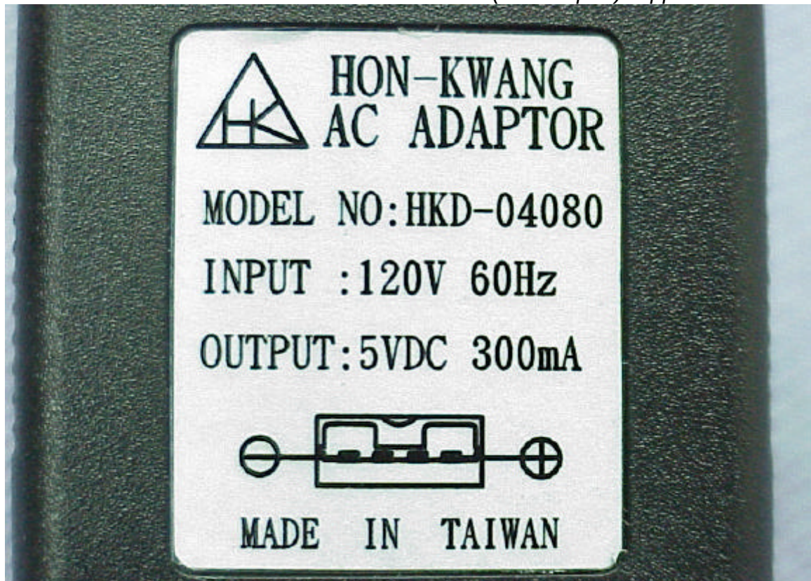
Photo 8 (AC Adapter) Appearance View/Label
