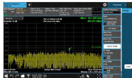
Band41-10MHz-QPSK-41540-1RB#49-0.009~0.15-PASS
