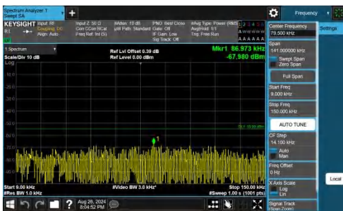
Band41-10MHz-QPSK-39700-1RB#0-0.009~0.15-PASS
