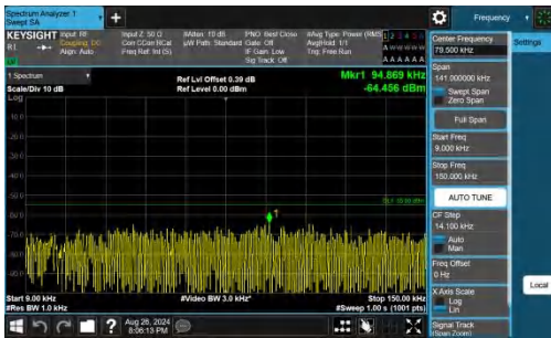
Band41-10MHz-QPSK-40620-1RB#0-0.009~0.15-PASS
