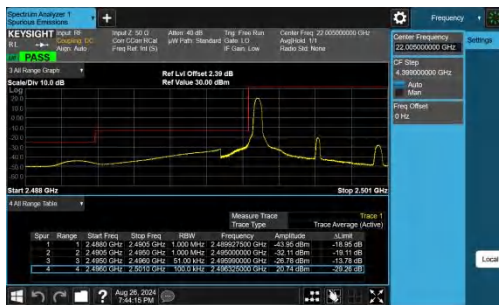
Band41-5MHz-QPSK-39675-1RB#0-PASS
