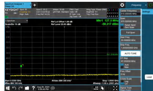
Band41-20MHz-QPSK-41490-1RB#99-30~1000-PASS
