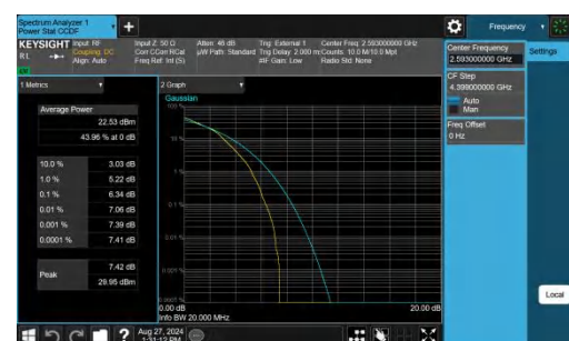
Band41-20MHz-16QAM-40620-27RB#0-PASS
