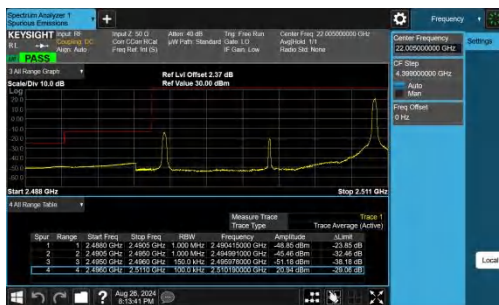
Band41-15MHz-QPSK-39725-1RB#74-PASS
