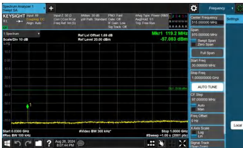
Band41-10MHz-QPSK-41540-1RB#0-30~1000-PASS
