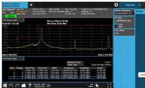
Band41-20MHz-QPSK-39750-1RB#0-PASS
