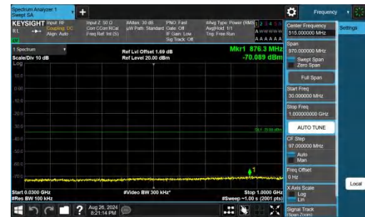
Band41-15MHz-QPSK-40620-1RB#74-30~1000-PASS
