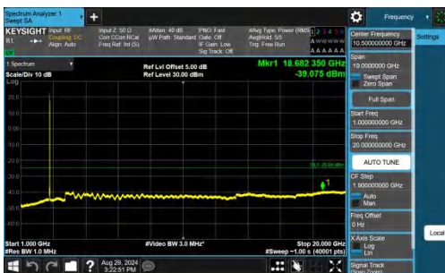
Band41-20MHz-QPSK-41490-1RB#99-1000~20000-PASS
