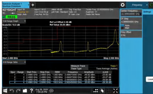
Band41-10MHz-QPSK-39700-1RB#49-PASS
