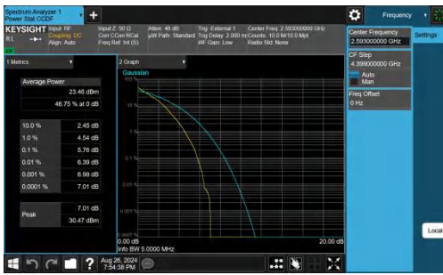
Band41-5MHz-QPSK-40620-25RB#0-PASS
