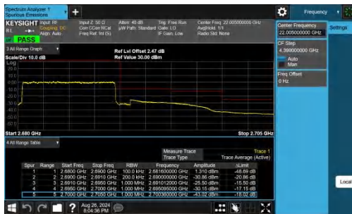
Band41-10MHz-QPSK-41540-50RB#0-PASS
