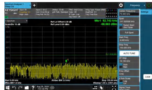
Band41-5MHz-QPSK-39675-1RB#24-0.009~0.15-PASS
