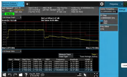
Band41-15MHz-QPSK-41515-75RB#0-PASS
