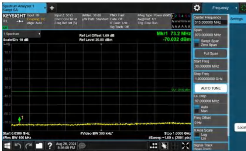
Band41-20MHz-QPSK-41490-1RB#0-30~1000-PASS
