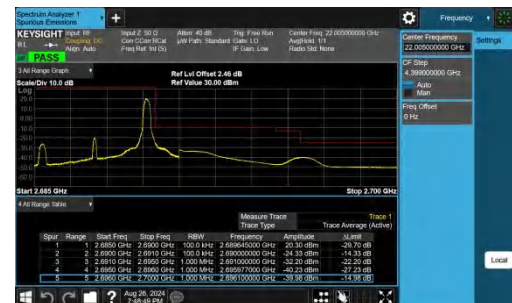
Band41-5MHz-QPSK-41565-1RB#24-PASS
