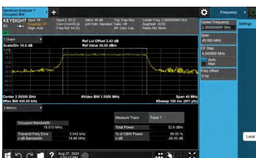
Band41-20MHz-QPSK-40620-100RB#0-PASS
