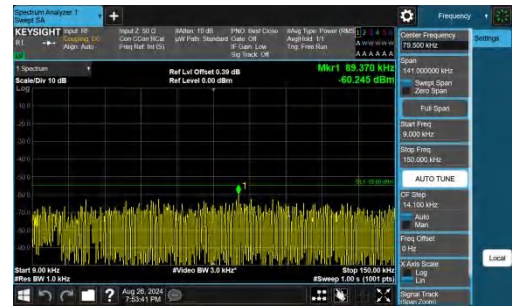
Band41-5MHz-QPSK-41565-1RB#24-0.009~0.15-PASS
