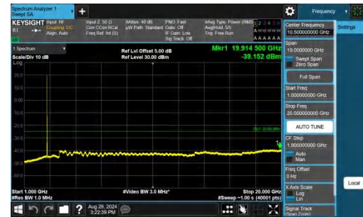
Band41-20MHz-QPSK-41490-1RB#0-1000~20000-PASS
