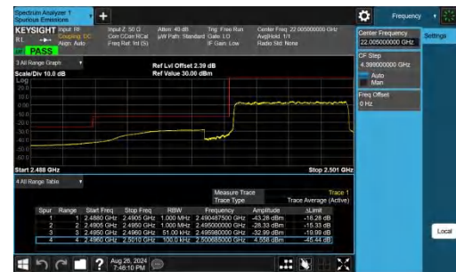
Band41-5MHz-QPSK-39675-25RB#0-PASS
