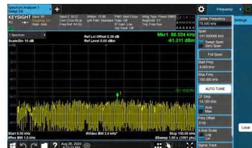
Band41-15MHz-QPSK-41515-1RB#74-0.009~0.15-PASS
