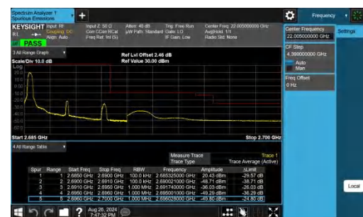
Band41-5MHz-QPSK-41565-1RB#0-PASS
