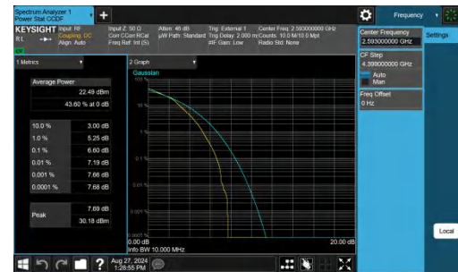
Band41-10MHz-16QAM-40620-27RB#0-PASS
