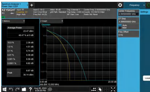
Band41-10MHz-QPSK-40620-50RB#0-PASS
