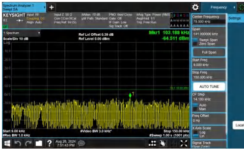
Band41-5MHz-QPSK-40620-1RB#0-0.009~0.15-PASS
