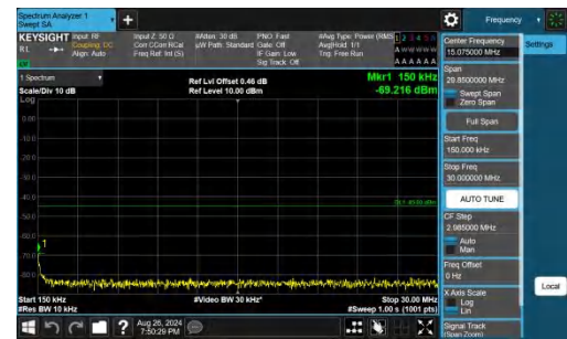
Band41-5MHz-QPSK-39675-1RB#0-0.15~30-PASS
