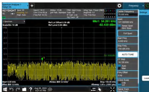
Band41-15MHz-QPSK-41515-1RB#0-0.009~0.15-PASS
