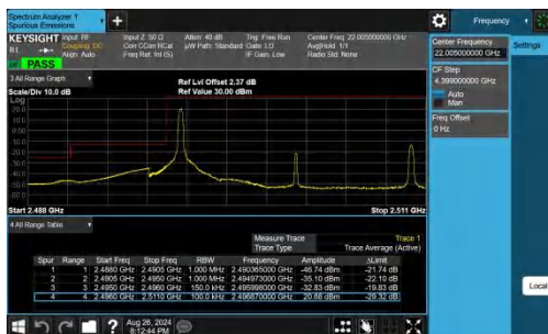
Band41-15MHz-QPSK-39725-1RB#0-PASS
