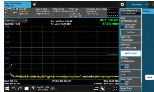
Band41-10MHz-QPSK-41540-1RB#0-0.15~30-PASS
