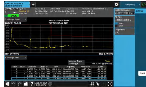
Band41-10MHz-QPSK-41540-1RB#0-PASS
