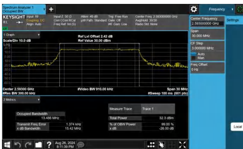
Band41-15MHz-QPSK-40620-75RB#0-PASS
