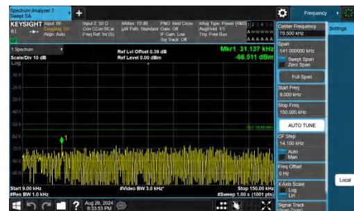
Band41-20MHz-QPSK-39750-1RB#99-0.009~0.15-PASS
