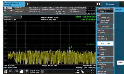
Band41-10MHz-QPSK-40620-1RB#49-0.009~0.15-PASS
