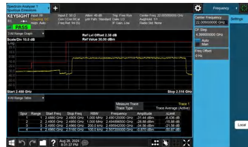
Band41-20MHz-QPSK-39750-100RB#0-PASS
