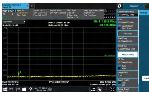
Band41-5MHz-QPSK-39675-1RB#0-30~1000-PASS
