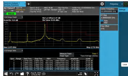
Band41-15MHz-QPSK-41515-1RB#74-PASS
