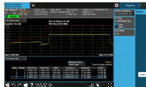
Band41-15MHz-QPSK-39725-75RB#0-PASS
