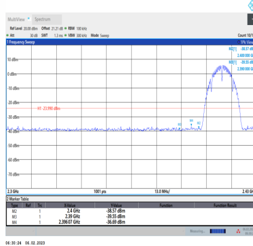
11B-Ant1-Low-2412-6.01
