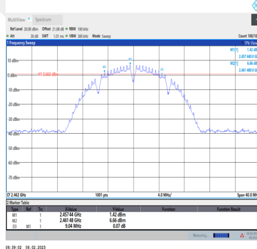
11B-Ant1-2462
