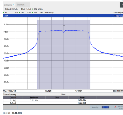
11G-Ant1-2412-NA-----15.81-94.09-0.26
