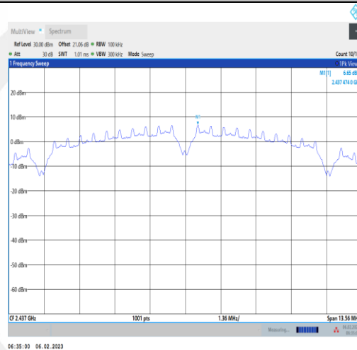
11B-Ant1-2437-2437.47
