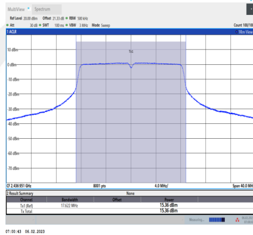
11G-Ant1-2437-NA-----15.09-94.06-0.27
