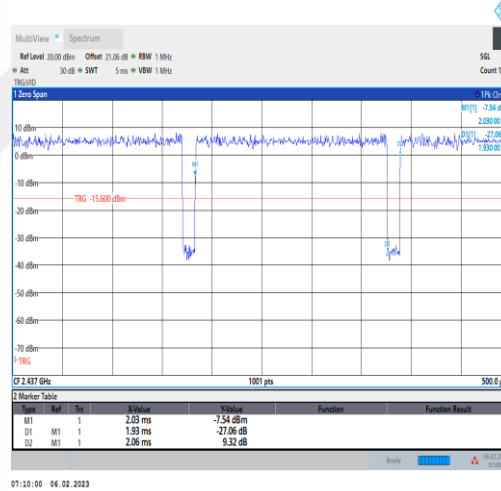
NTNV-11N20SISO-Ant1-2437
