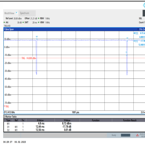
NTNV-11B-Ant1-2412
