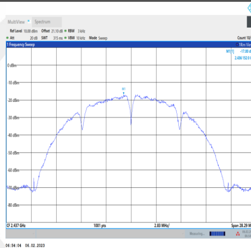
11B-Ant1-2437--17.04-0.04-0.00-0.00
