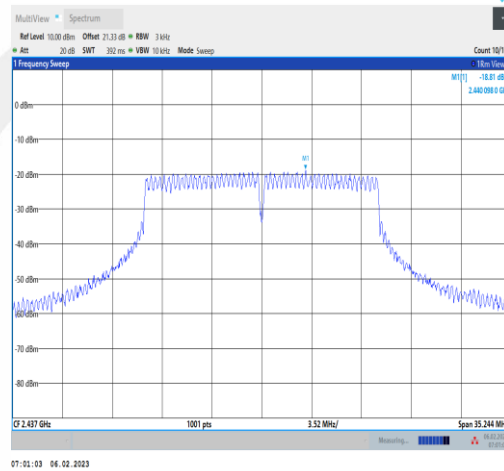
11G-Ant1-2437--19.08-0.27-0.00-0.00
