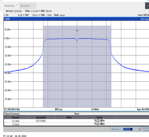
11N20SISO-Ant1-2462-NA-----13.94-93.66-0.28
