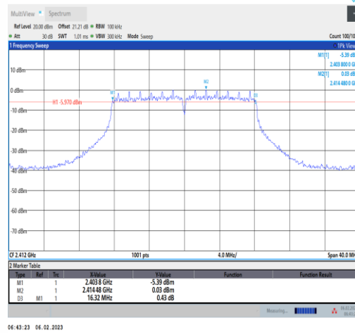
11G-Ant1-2412
