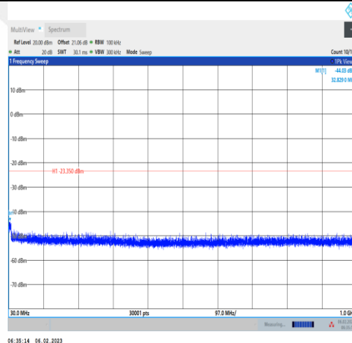
11B-Ant1-2437-30~1000-6.65
