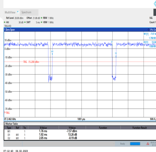
NTNV-11N20SISO-Ant1-2462
