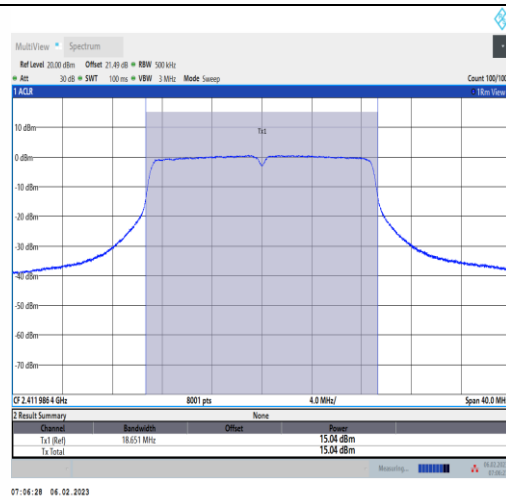
11N20SISO-Ant1-2412-NA-----14.76-93.66-0.28
