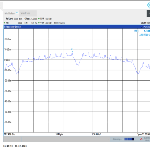
11B-Ant1-2462-2461.47
