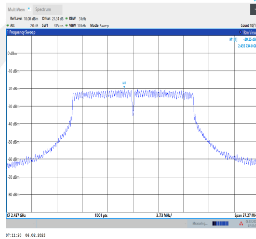
11N20SISO-Ant1-2437--20.53-0.28-0.00-0.00
