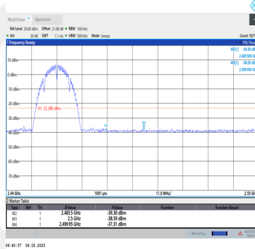
11B-Ant1-High-2462-6.72
