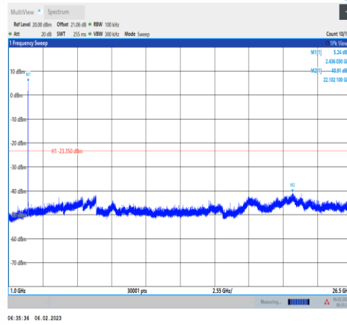
11B-Ant1-2437-1000~26500-6.65
