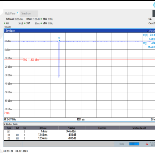
NTNV-11B-Ant1-2437
