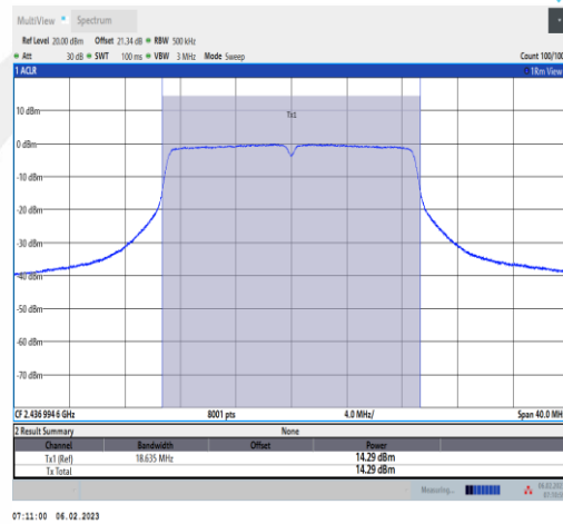
11N20SISO-Ant1-2437-NA-----14.01-93.69-0.28
