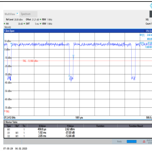
NTNV-11N20SISO-Ant1-2412
