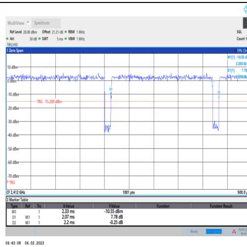
NTNV-11G-Ant1-2412
