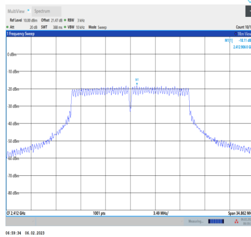
11G-Ant1-2412--18.37-0.26-0.00-0.00
