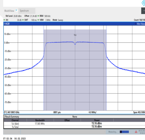
11G-Ant1-2462-NA-----14.90-94.09-0.26
