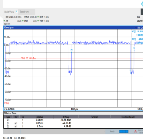
NTNV-11G-Ant1-2462
