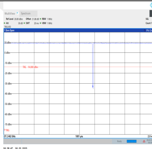
NTNV-11B-Ant1-2462
