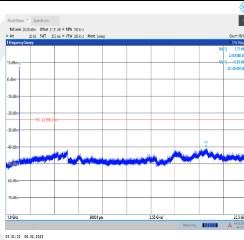
11B-Ant1-2412-1000~26500-6.01
