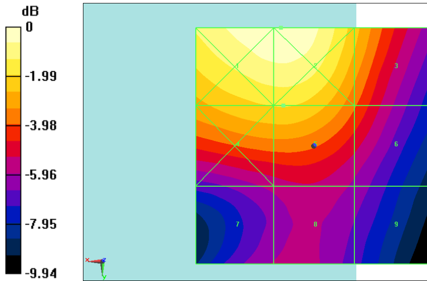
Fig B.2 HAC RF E-Field LTE Band41 QPSK PC2
