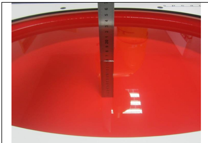
Liquid depth in the flat Phantom
