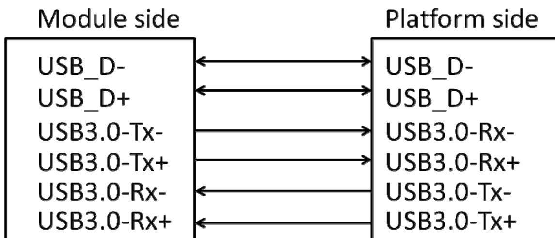
Figure 1-3 USB3.0 interface.
