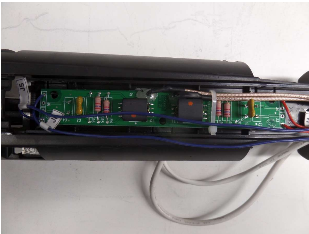
Figure 11: NS40 antenna A1200 matching coupler board top side
