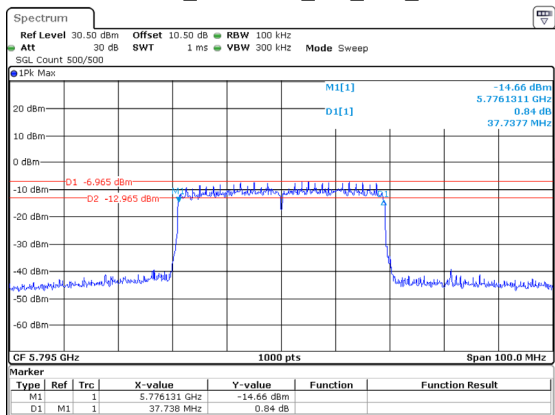
802.11ax40_5795MHz_RU_Full_Chain 2
