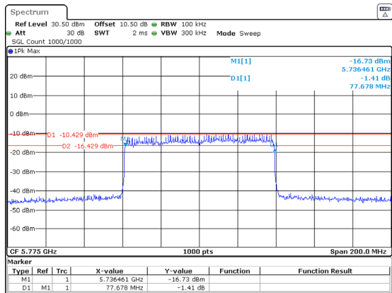
802.11ax80_5775MHz_RU_Full_Chain 1
