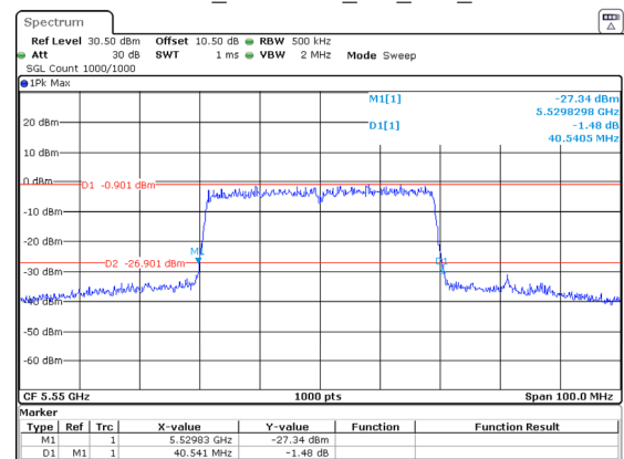
802.11ax40_5550MHz_RU_Full_Chain 1
