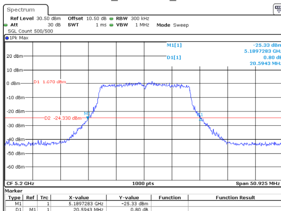
802.11a_5200MHz_Chain 2
