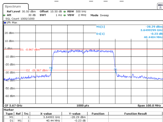
802.11ax40_5670MHz_RU_Full_Chain 1
