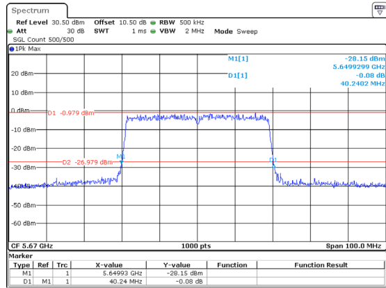
802.11ax40_5670MHz_RU_Full_Chain 2
