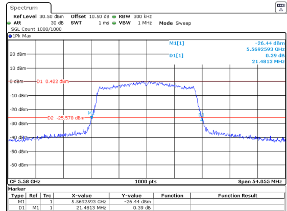
802.11ax20_5580MHz_RU_Full_Chain 1
