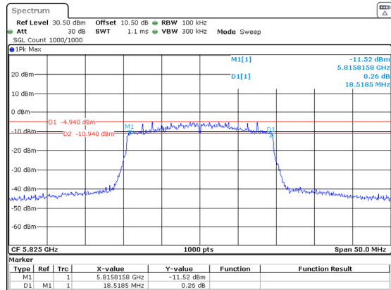
802.11ax20_5825MHz_RU_Full_Chain 1
