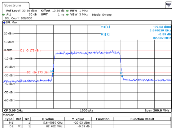
802.11ax80_5690MHz_RU_Full_Chain 2
