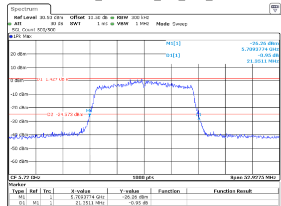
802.11ax20_5720MHz_RU_Full_Chain 2
