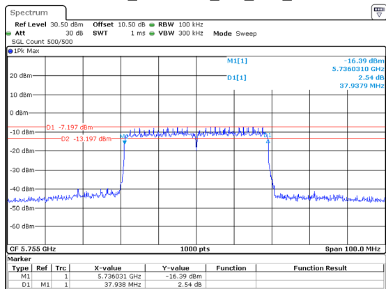
802.11ax40_5755MHz_RU_Full_Chain 2
