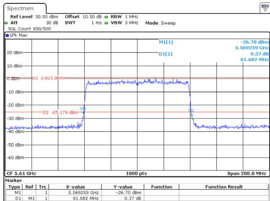
802.11ax80_5610MHz_RU_Full_Chain 2
