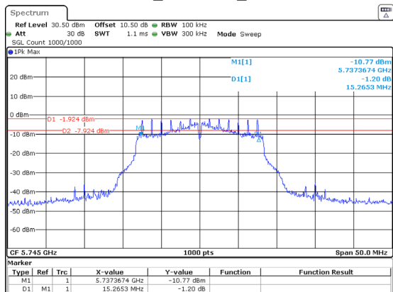
802.11a_5745MHz_Chain 1
