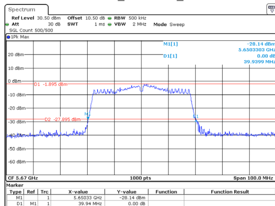
802.11ac40_5670MHz_Chain 2
