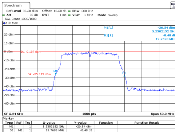
802.11a_5240MHz_Chain 1
