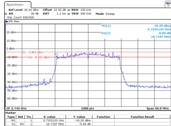
802.11ax20_5745MHz_RU_Full_Chain 2
