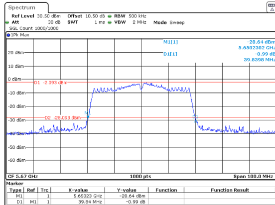
802.11ac40_5670MHz_Chain 1
