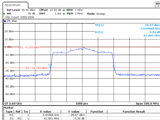
802.11ac80_5690MHz_Chain 1
