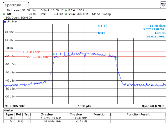
802.11ax20_5785MHz_RU_Full_Chain 2
