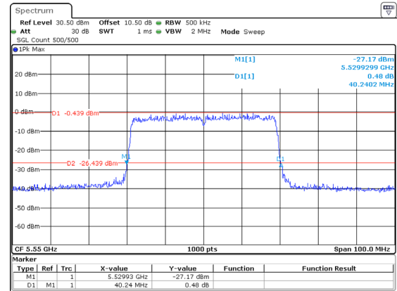
802.11ax40_5550MHz_RU_Full_Chain 2
