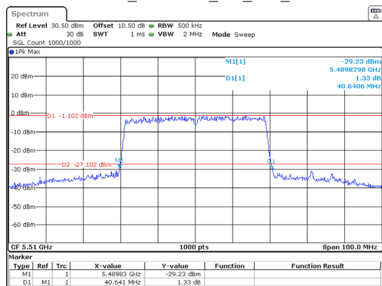
802.11ax40_5510MHz_RU_Full_Chain 1
