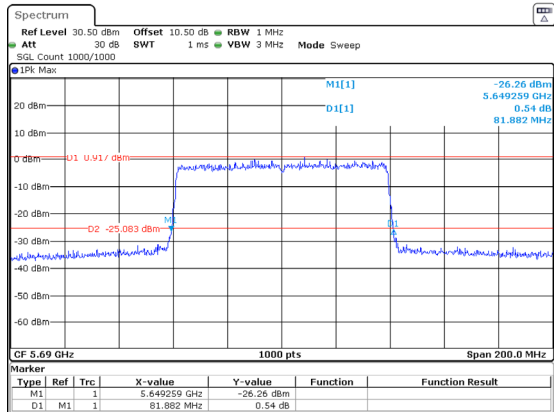
802.11ax80_5690MHz_RU_Full_Chain 1
