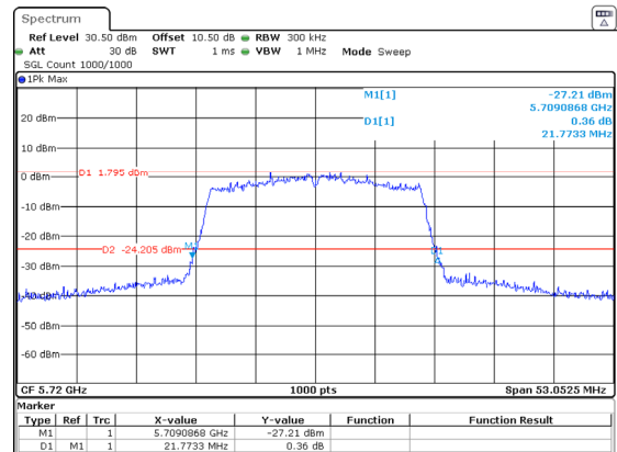
802.11ax20_5720MHz_RU_Full_Chain 1
