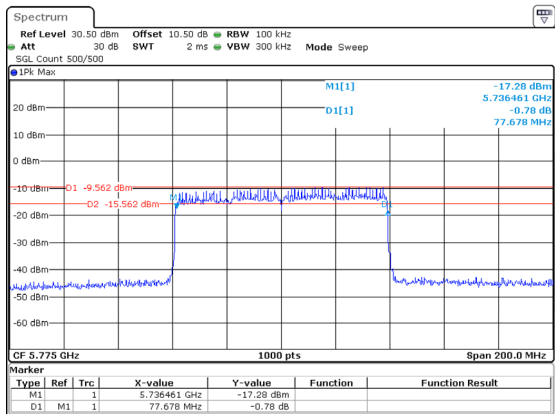
802.11ax80_5775MHz_RU_Full_Chain 2
