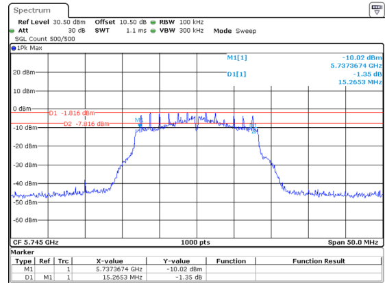
802.11a_5745MHz_Chain 2
