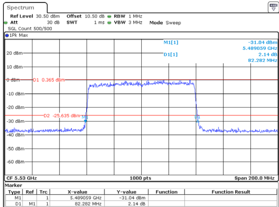
802.11ax80_5530MHz_RU_Full_Chain 2
