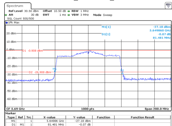
802.11ac80_5690MHz_Chain 2
