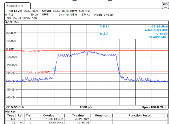
802.11ac40_5550MHz_Chain 1
