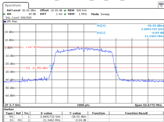
802.11ax20_5700MHz_RU_Full_Chain 2
