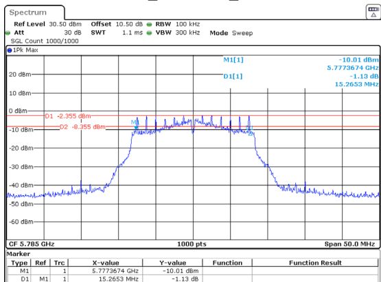
802.11a_5785MHz_Chain 1
