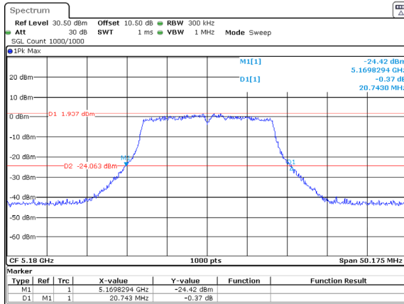
802.11a_5180MHz_Chain 1
