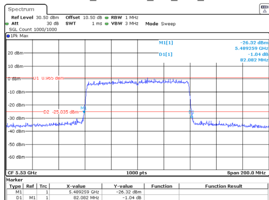
802.11ax80_5530MHz_RU_Full_Chain 1
