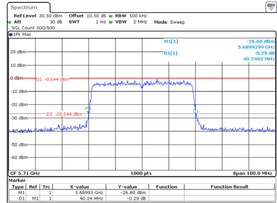
802.11ax40_5710MHz_RU_Full_Chain 2
