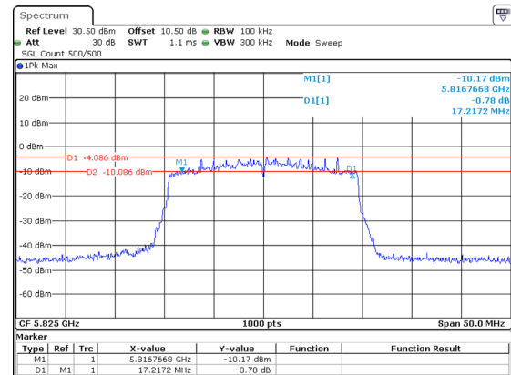
802.11ax20_5825MHz_RU_Full_Chain 2
