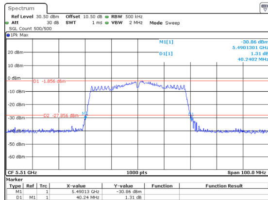
802.11ac40_5510MHz_Chain 2
