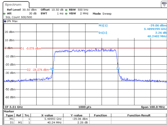
802.11ax40_5510MHz_RU_Full_Chain 2
