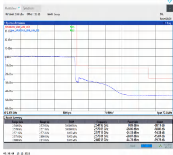
1-N7-15-30-H-6-CP-QPSK-Outer_Full-160@0-Ant1-1--PASS-see graph
