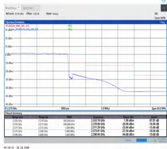
1-N7-15-20-H-6-CP-QPSK-Outer_Full-106@0-Ant1-1--PASS-see graph
