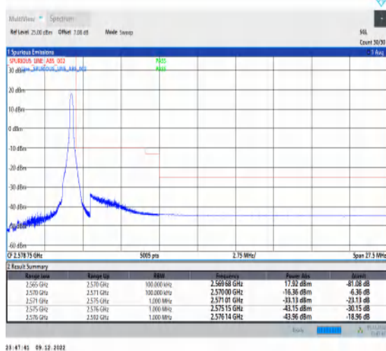
1-N7-15-5-H-5-CP-QPSK-Edge_1RB_Right-1@24-Ant1-1--PASS-see graph
