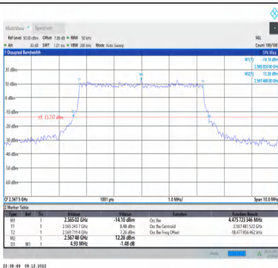
1-N7-15-5-H-3-DFT-16QAM-Outer_Full-25@0-Ant1-4.476-4.930-≤5-PASS
