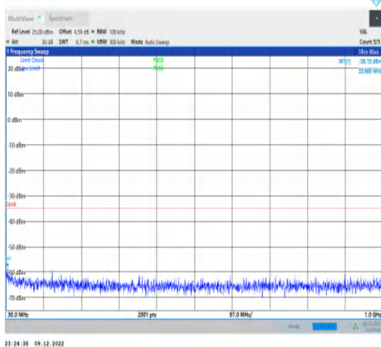
1-N7-15-40-H-1-DFT-PI2BPSK-Inner_1RB_Left-1@ 1-30-1000-Ant1-33.88--58.15--35-PASS
