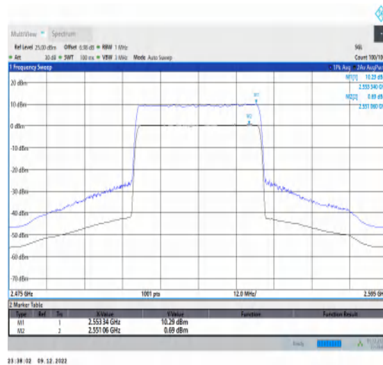
1-N7-15-40-M-2-CP-256QAM-Outer_Full-216@0-Ant t1-9.60-100%-0.00-9.60-PASS-≤13
