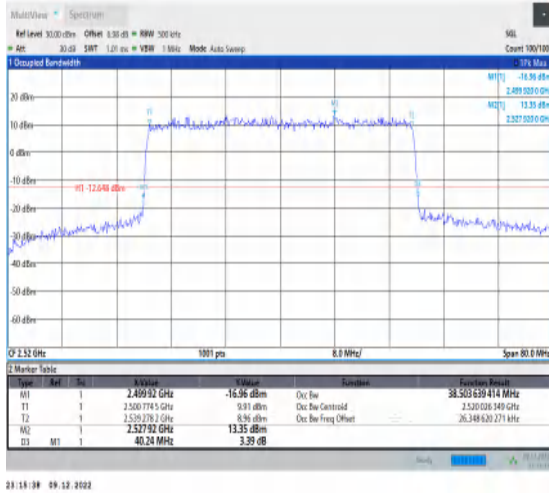
1-N7-15-40-L-3-DFT-16QAM-Outer_Full-216@0-Ant 1-38.504-40.240-≤40-PASS
