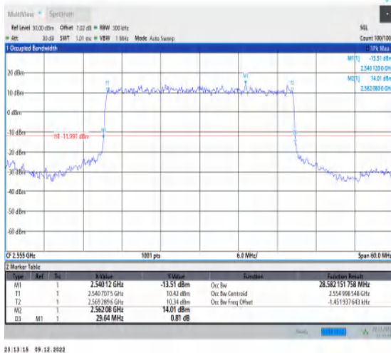
1-N7-15-30-H-2-DFT-P12BPSK-Outer_Full-160@0-A nt1-28.582-29.640-≤30-PASS
