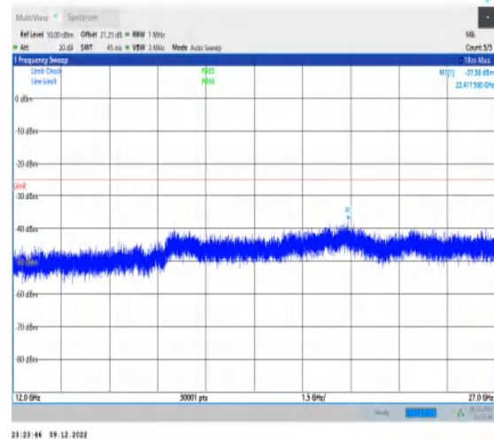
1-N7-15-40-M-1-DFT-PI2BPSK-Inner_1RB_Left-1@ -12000-27000-Ant1-22417.50--37.58--25-PASS
