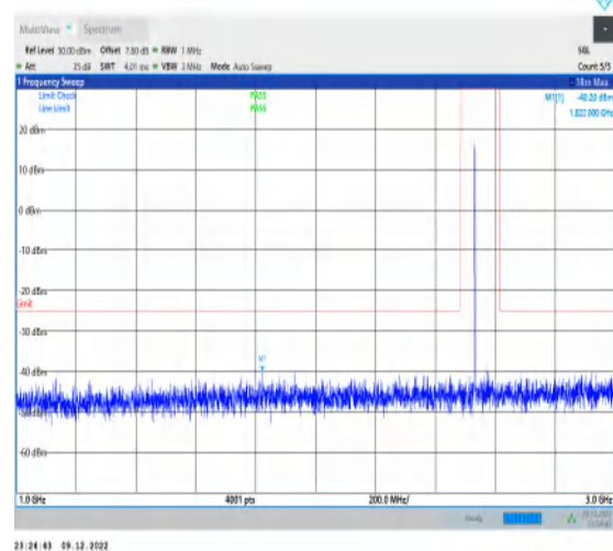
1-N7-15-40-H-1-DFT-PI2BPSK-Inner_1RB_Left-1@ -1000-3000-Ant1-1822.00--40.20--25-PASS
