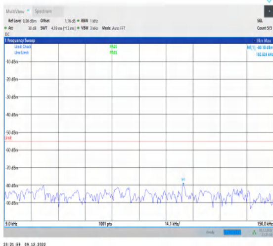
1-N7-15-40-L-1-DFT-PI2BPSK-Inner_1RB_Left-1@ 1-0.009-0.15-Ant1-0.10--80.18--55-PASS
