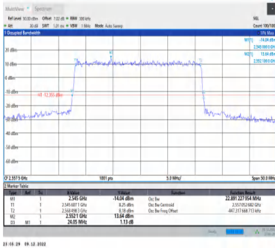
1-N7-15-25-H-3-DFT-16QAM-Outer_Full-128@0-Ant 1-22.891-24.050-≤25-PASS
