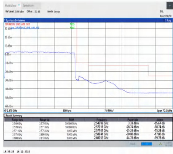
1-N7-15-30-H-3-DFT-PI2BPSK-Outer_Full-160@0-Ant1-1--PASS-see graph
