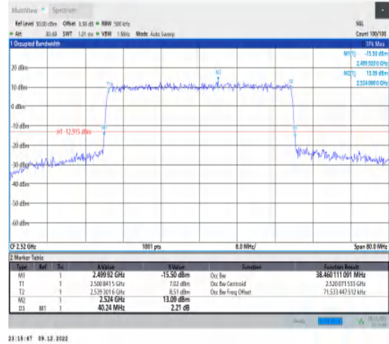
1-N7-15-40-L-4-DFT-64QAM-Outer_Full-216@0-Ant 1-38.46-40.240-≤40-PASS
