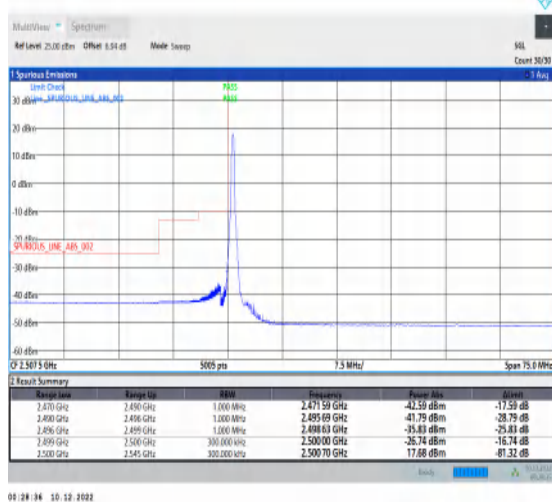
1-N7-15-30-L-4-CP-QPSK-Edge_1RB_Left-1@0-Ant1-1--PASS-see graph
