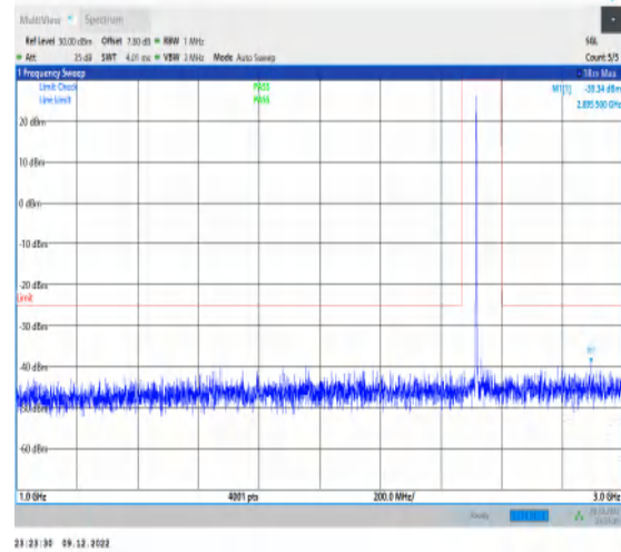
1-N7-15-40-M-1-DFT-PI2BPSK-Inner_1RB_Left-1@ -1000-3000-Ant1-2895.50--39.34--25-PASS
