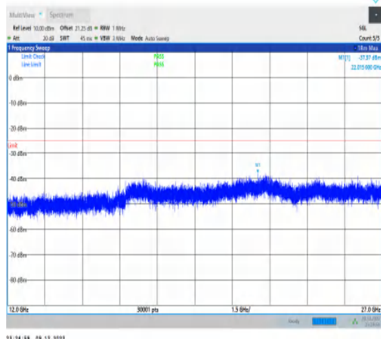
1-N7-15-40-H-1-DFT-PI2BPSK-Inner_1RB_Left-1@ -12000-27000-Ant1-22015.00--37.97--25-PASS
