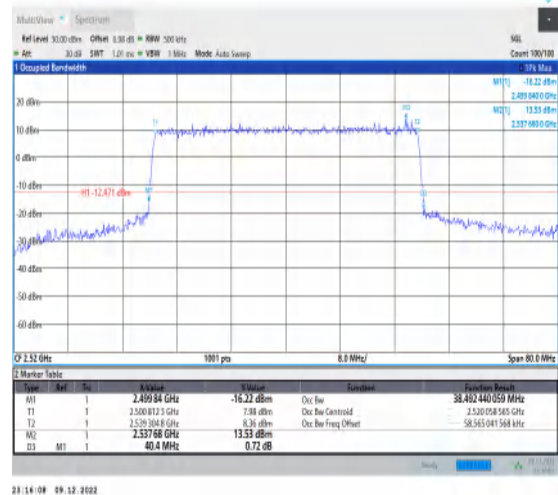
1-N7-15-40-L-6-CP-QPSK-Outer_Full-216@0-Ant1-3 8.492-40.400-≤40-PASS
