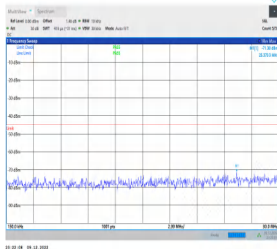
1-N7-15-40-L-1-DFT-PI2BPSK-Inner_1RB_Left-1@1- 0.15-30-Ant1-25.37--71.30--45-PASS
