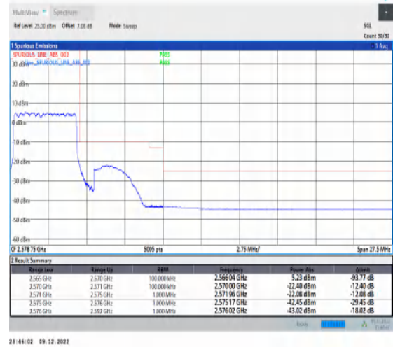
1-N7-15-5-H-3-DFT-PI2BPSK-Outer_Full-25@0-Ant1-1--PASS-see graph
