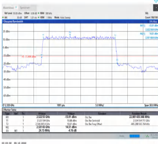
1-N7-15-25-M-2-DFT-PI2BPSK-Outer_Full-128@0-A nt1-22.901-24.150-≤25-PASS
