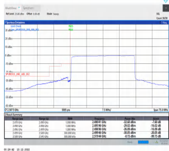
1-N7-15-30-L-6-CP-QPSK-Outer_Full-160@0-Ant1-1--PASS-see graph
