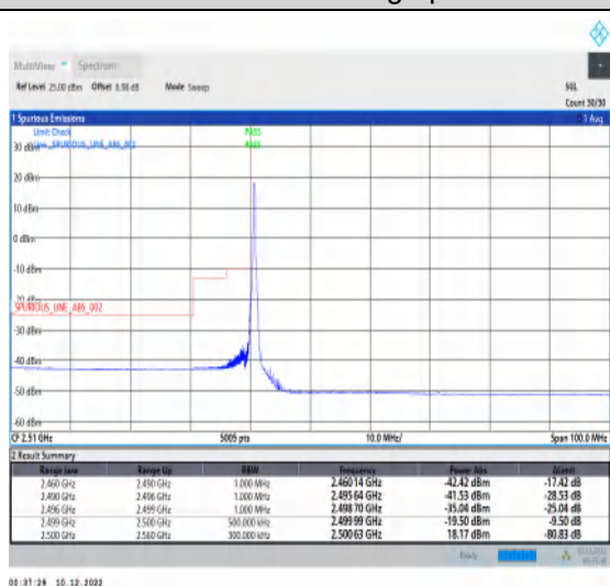
1-N7-15-40-L-4-CP-QPSK-Edge_1RB_Left-1@0-Ant1-1--PASS-see graph
