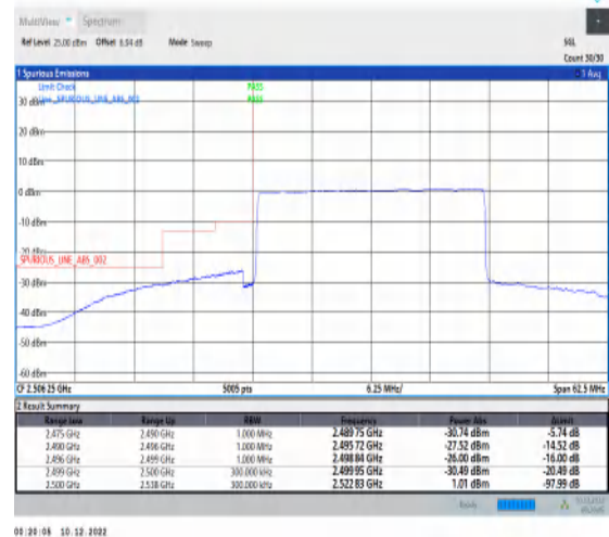
1-N7-15-25-L-6-CP-QPSK-Outer_Full-133@0-Ant1-1--PASS-see graph
