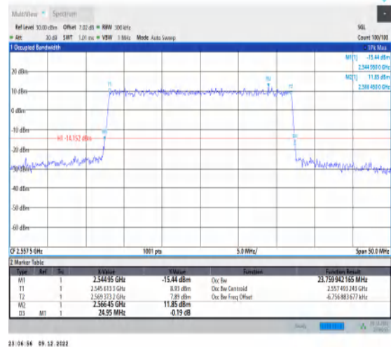
1-N7-15-25-H-6-CP-QPSK-Outer_Full-133@0-Ant1 23.76-24.950-≤25-PASS
