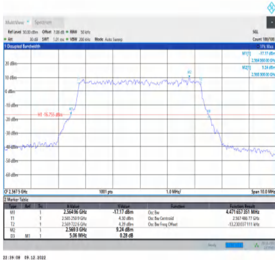
1-N7-15-5-H-5-DFT-256QAM-Outer_Full-25@0-Ant1-4.472-5.060-≤5-PASS
