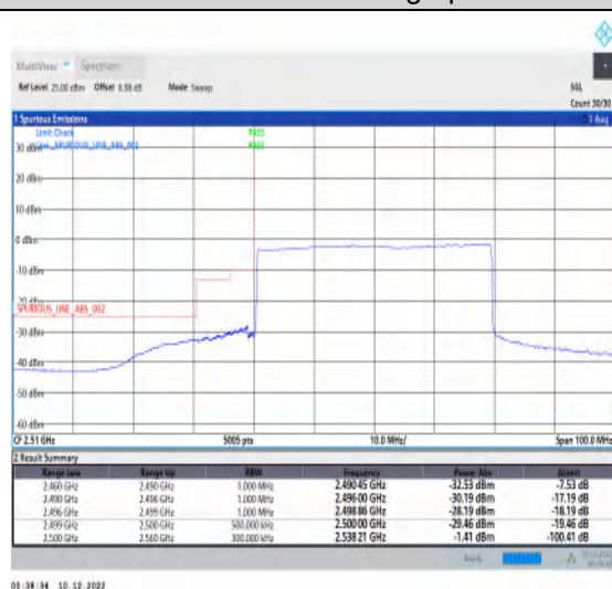
1-N7-15-40-L-6-CP-QPSK-Outer_Full-216@0-Ant1-1--PASS-see graph
