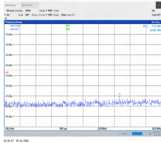
1-N7-15-40-H-1-DFT-PI2BPSK-Inner_1RB_Left-1@ -0.15-30-Ant1-22.03--71.61--45-PASS
