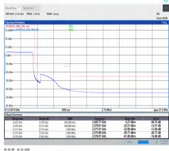
1-N7-15-5-H-6-CP-QPSK-Outer_Full-25@0-Ant1-1--PASS-see graph
