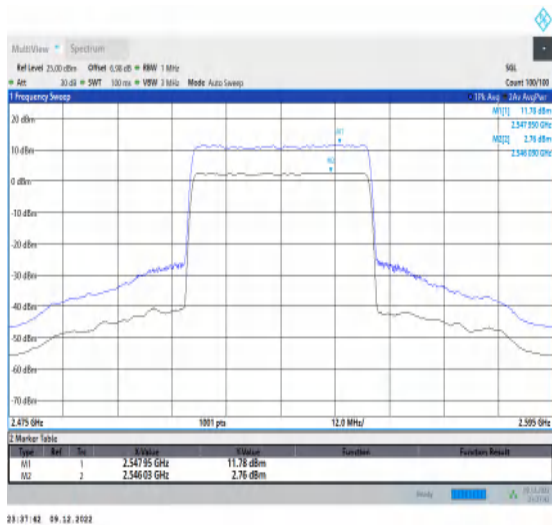
1-N7-15-40-M-1-DFT-256QAM-Outer_Full-216@0-Ant nt1-9.02-100%-0.00-9.02-PASS-≤13
