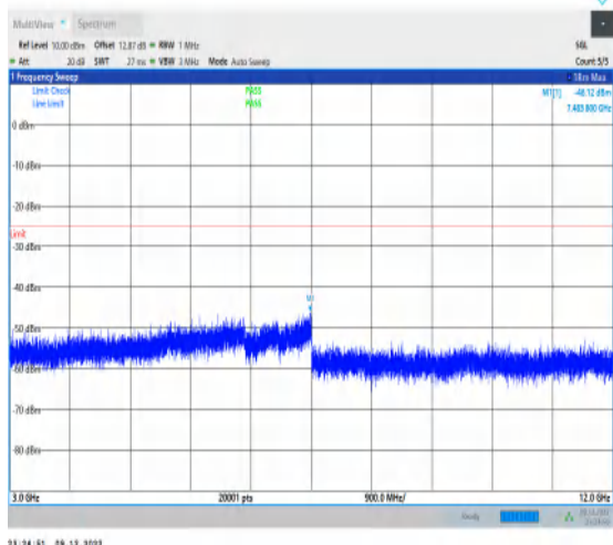
1-N7-15-40-H-1-DFT-PI2BPSK-Inner_1RB_Left-1@ 1-3000-12000-Ant1-7483.80--46.12--25-PASS
