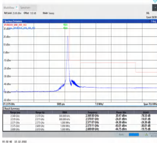
1-N7-15-30-H-5-CP-QPSK-Edge_1RB_Right-1@159-Ant1-1--PASS-see graph
