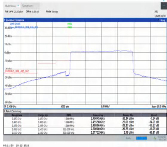
1-N7-15-20-L-6-CP-QPSK-Outer_Full-106@0-Ant1-1--PASS-see graph
