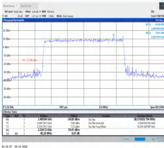
1-N7-15-40-L-5-DFT-256QAM-Outer_Full-216@0-Ant t1-38.52-40.240-≤40-PASS
