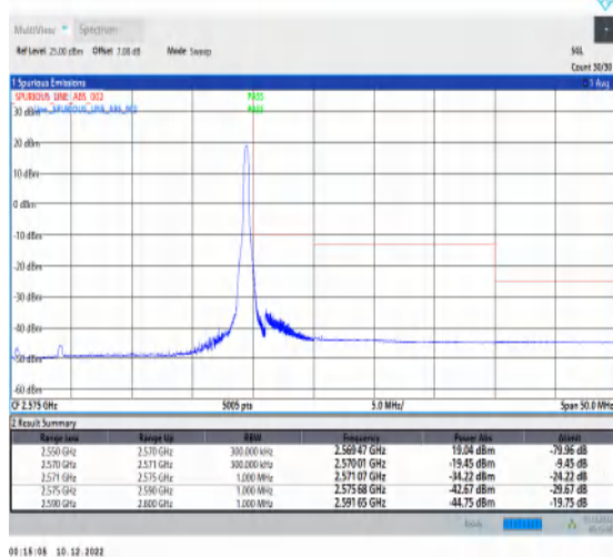
1-N7-15-20-H-5-CP-QPSK-Edge_1RB_Right-1@105-Ant1-1--PASS-see graph
