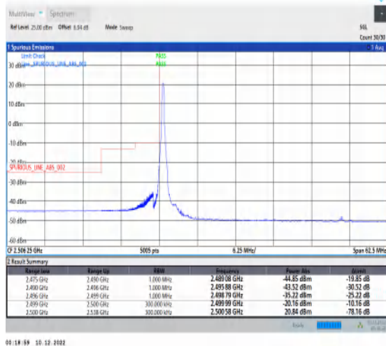
1-N7-15-25-L-4-CP-QPSK-Edge_1RB_Left-1@0-Ant1-1--PASS-see graph
