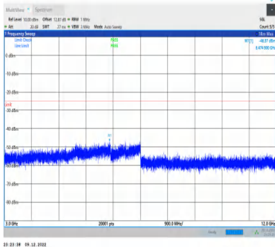
1-N7-15-40-M-1-DFT-PI2BPSK-Inner_1RB_Left-1@ 1-3000-12000-Ant1-6474.90--46.97--25-PASS
