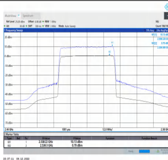
1-N7-15-40-L-2-CP-256QAM-Outer_Full-216@0-Ant 1-9.43-100%-0.00-9.43-PASS-≤13
