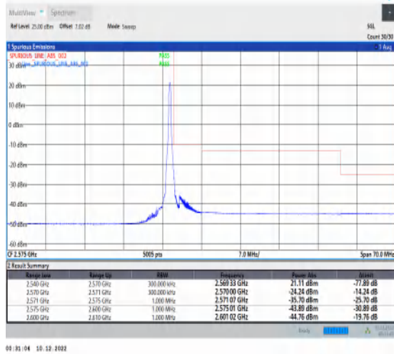
1-N7-15-30-H-2-DFT-PI2BPSK-Edge_1RB_Right-1@159-Ant1-1--PASS-see graph
