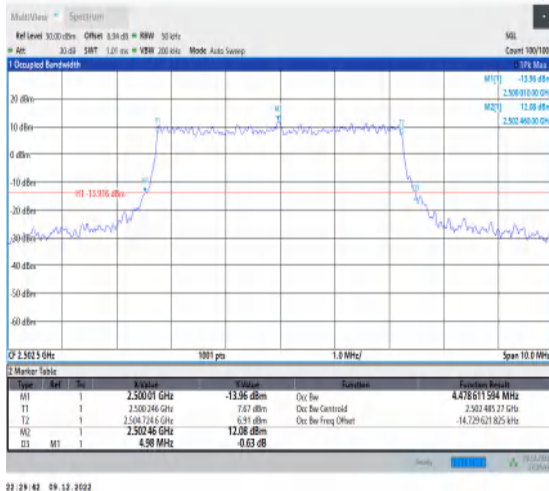
1-N7-15-5-L-3-DFT-16QAM-Outer_Full-25@0-Ant1-4 .479-4.980-≤5-PASS
