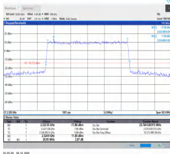
1-N7-15-25-M-3-DFT-16QAM-Outer_Full-128@0-Ant 1-22.993-24.000-≤25-PASS
