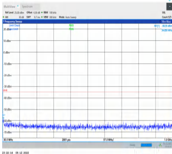
1-N7-15-40-L-1-DFT-PI2BPSK-Inner_1RB_Left-1@ 1-30-1000-Ant1-34.85--58.55--35-PASS
