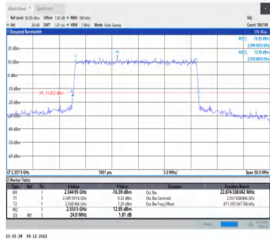
1-N7-15-25-H-4-DFT-64QAM-Outer_Full-128@0-Ant 1-22.874-24.000-≤25-PASS
