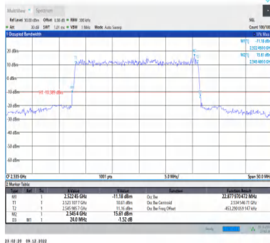
1-N7-15-25-M-1-DFT-QPSK-Outer_Full-128@0-Ant1 -22.878-24.000-≤25-PASS
