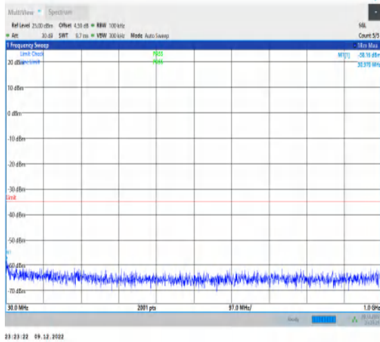
1-N7-15-40-M-1-DFT-PI2BPSK-Inner_1RB_Left-1@ 1-30-1000-Ant1-30.97--58.16--35-PASS
