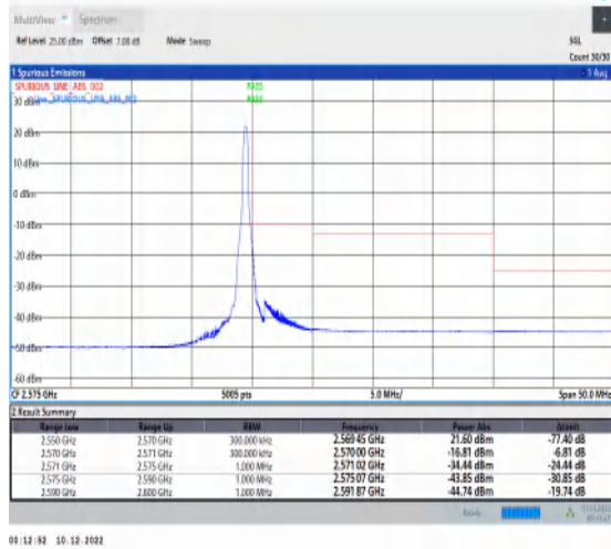
1-N7-15-20-H-2-DFT-PI2BPSK-Edge_1RB_Right-1@105-Ant1-1--PASS-see graph
