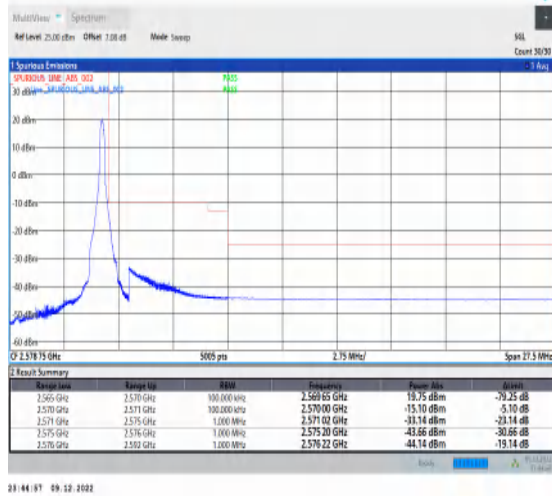
1-N7-15-5-H-2-DFT-PI2BPSK-Edge_1RB_Right-1@24-Ant1-1--PASS-see graph
