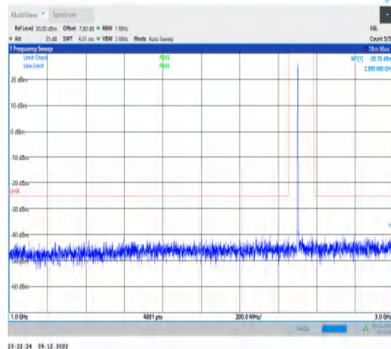
1-N7-15-40-L-1-DFT-PI2BPSK-Inner_1RB_Left-1@1- 1000-3000-Ant1-2999.00--39.70--25-PASS
