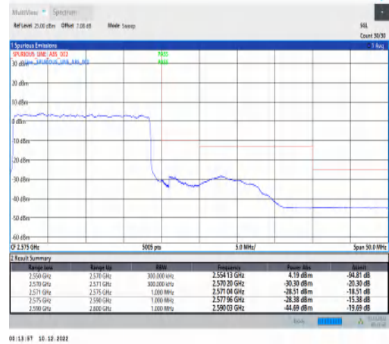
1-N7-15-20-H-3-DFT-PI2BPSK-Outer_Full-100@0-Ant1-1--PASS-see graph
