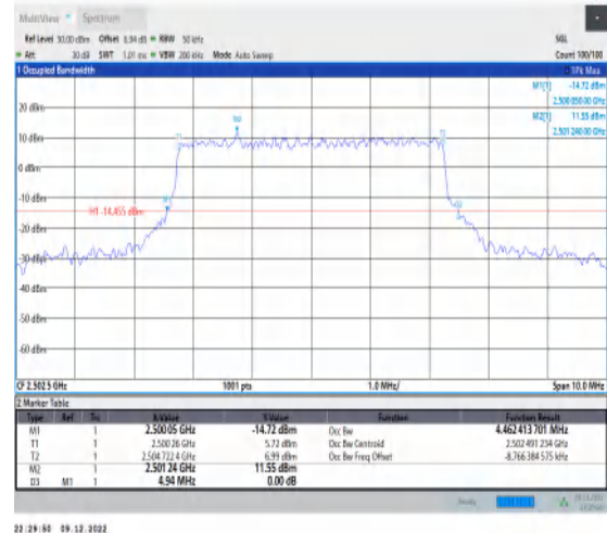
1-N7-15-5-L-4-DFT-64QAM-Outer_Full-25@0-Ant1-4 .462-4.940-≤5-PASS
