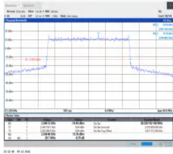
1-N7-15-30-H-1-DFT-QPSK-Outer_Full-160@0-Ant1 -28.55-29.700-≤30-PASS
