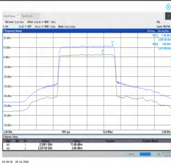
1-N7-15-40-L-1-DFT-256QAM-Outer_Full-216@0-Ant t1-9.08-100%-0.00-9.08-PASS-≤13
