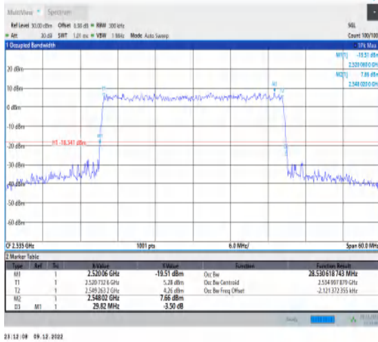
1-N7-15-30-M-9-CP-256QAM-Outer_Full-160@0-Ant 1-28.531-29.820-≤30-PASS
