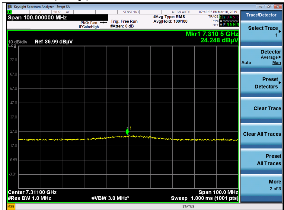
Middle channel 3 rd harmonic (Average)
