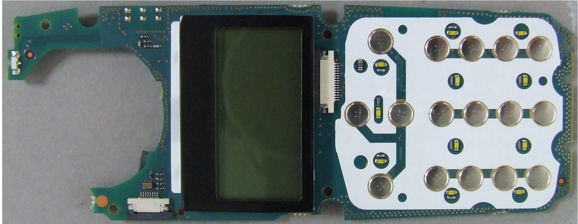
Photograph 05: Control PCB – top
