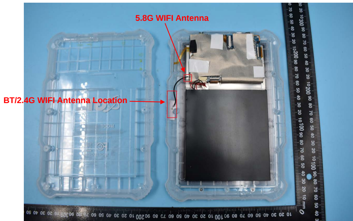
2. Antenna view
