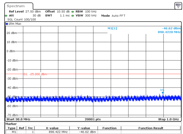
40MHz_30kHz_2600MHz_DFT-s-OFDM QPSK_RB100@0&amp;-46.62 dBm
