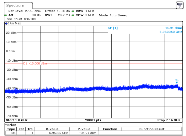
15MHz_15kHz_708.5MHz_DFT-s-OFDM QPSK_RB1@0&amp;-34.91 dBm
