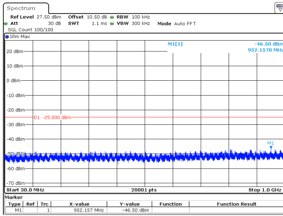
15MHz_30kHz_2595MHz_DFT-s-OFDM QPSK_RB1@0&amp;-46.50 dBm
