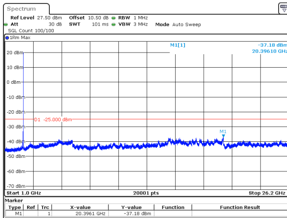
40MHz_30kHz_2600MHz_DFT-s-OFDM QPSK_RB1@105&amp;-37.18 dBm
