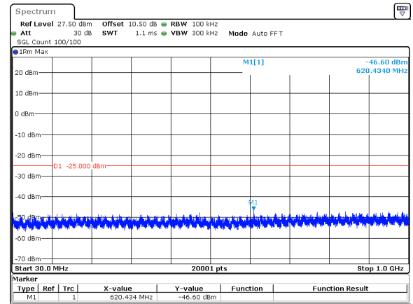
40MHz_30kHz_2600MHz_DFT-s-OFDM QPSK_RB1@0&amp;-46.60 dBm
