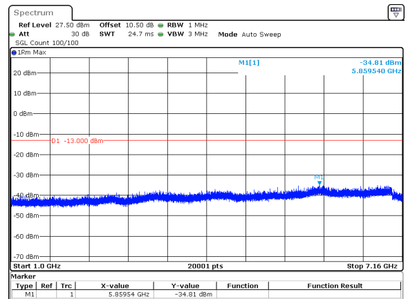
15MHz_15kHz_706.5MHz_DFT-s-OFDM QPSK_RB75@0&amp;-34.81 dBm
