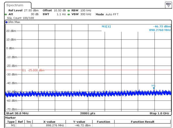
30MHz_30kHz_2595MHz_DFT-s-OFDM QPSK_RB1@77&amp;-46.72 dBm
