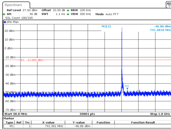
5MHz_15kHz_713.5MHz_DFT-s-OFDM QPSK_RB1@0&amp;-46.86 dBm
