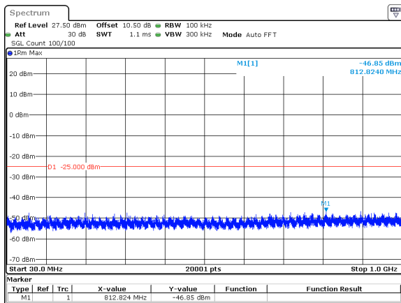
25MHz_30kHz_2582.5MHz_DFT-s-OFDM QPSK_RB1@64&amp;-46.85 dBm
