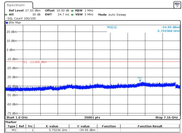
5MHz_15kHz_713.5MHz_DFT-s-OFDM QPSK_RB1@0&amp;-34.95 dBm
