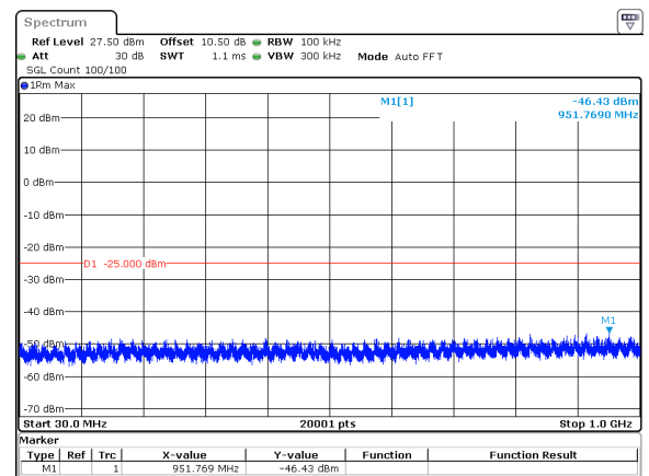
15MHz_30kHz_2577.5MHz_DFT-s-OFDM QPSK_RB36@0&amp;-46.43 dBm
