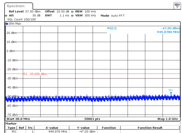
25MHz_30kHz_2595MHz_DFT-s-OFDM QPSK_RB64@0&amp;-47.03 dBm
