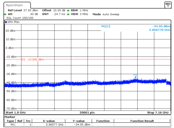
15MHz_15kHz_707.5MHz_DFT-s-OFDM QPSK_RB1@0&amp;-34.95 dBm
