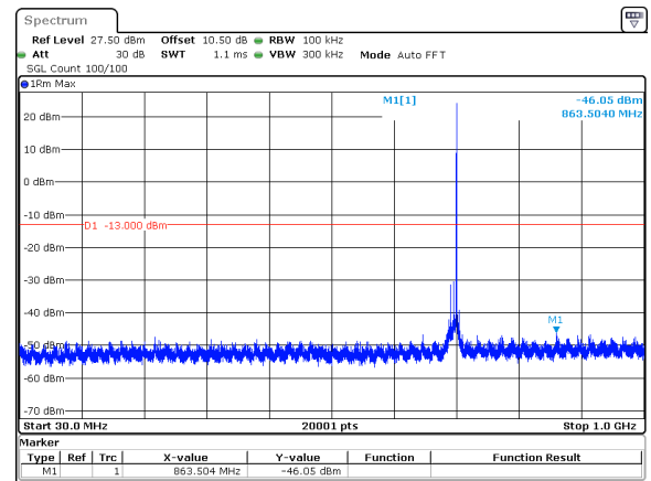
10MHz_15kHz_704MHz_DFT-s-OFDM QPSK_RB1@51&amp;-46.05 dBm
