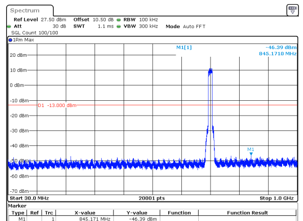
15MHz_15kHz_708.5MHz_DFT-s-OFDM QPSK_RB75@0&amp;-46.39 dBm
