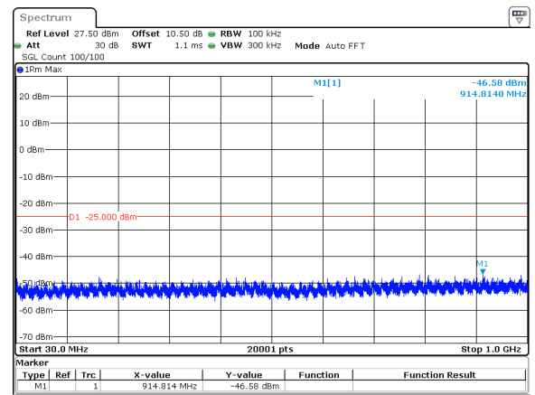
15MHz_30kHz_2612.5MHz_DFT-s-OFDM QPSK_RB1@0&amp;-46.58 dBm
