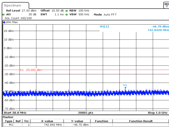
10MHz_15kHz_2593.005MHz_DFT-s-OFDM QPSK_RB1@51&amp;-46.70 dBm
