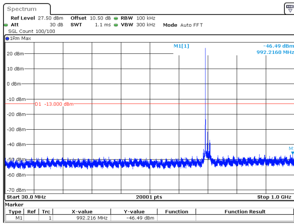
15MHz_15kHz_707.5MHz_DFT-s-OFDM QPSK_RB1@0&amp;-46.49 dBm
