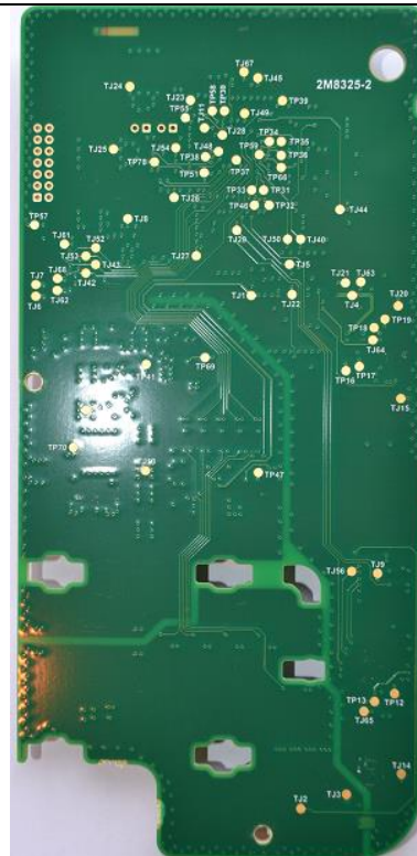
TWR-1 & TWR-5 Reader PCB Assy – Solder Side
