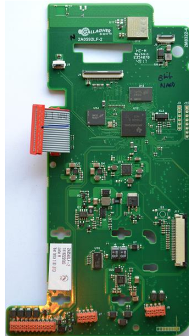
TWR-1 & TWR-5 WeighScale PCB Assy – Component Side
