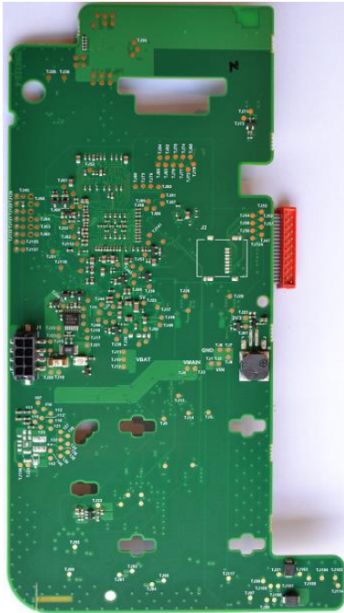
TWR-1 & TWR-5 WeighScale PCB Assy – Solder Side
