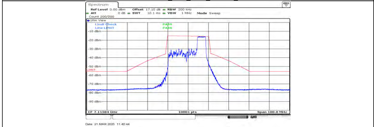
11AX20MIMO Ant1_7115_52Tone_RU40
