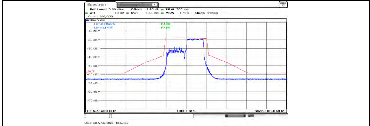
11AX20MIMO Ant1_6515_106Tone_RU54
