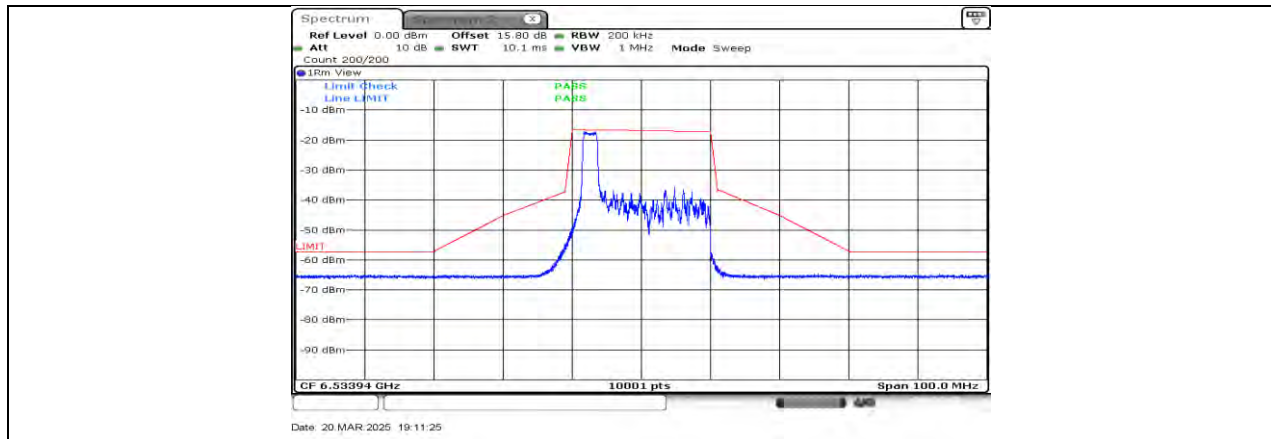
11AX20MIMO Ant1_6535_26Tone_RU0
