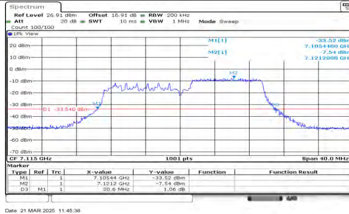
11AX20MIMO Ant2_7115_106Tone_RU54
