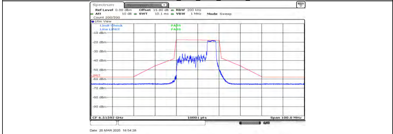
11AX20MIMO Ant1_6515_52Tone_RU40
