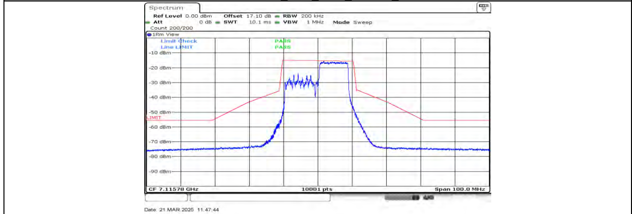
11AX20MIMO Ant1_7115_106Tone_RU54
