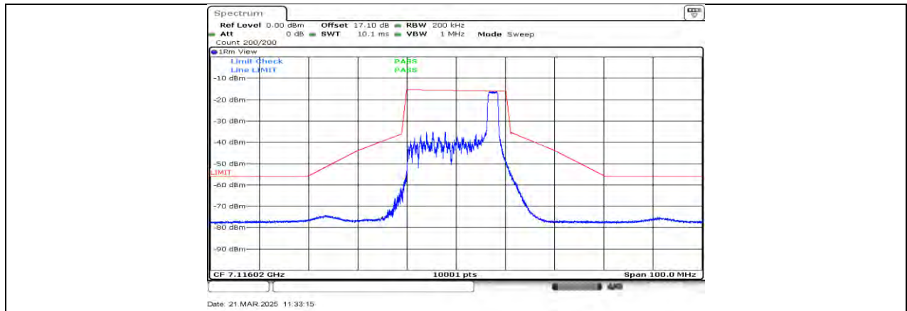
11AX20MIMO Ant1_7115_26Tone_RU8
