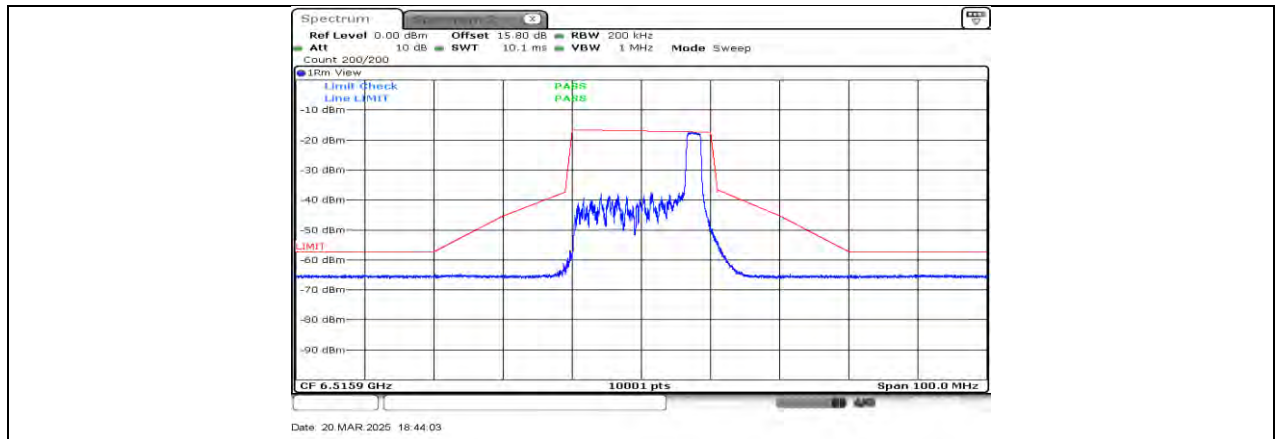
11AX20MIMO Ant1_6515_26Tone_RU8
