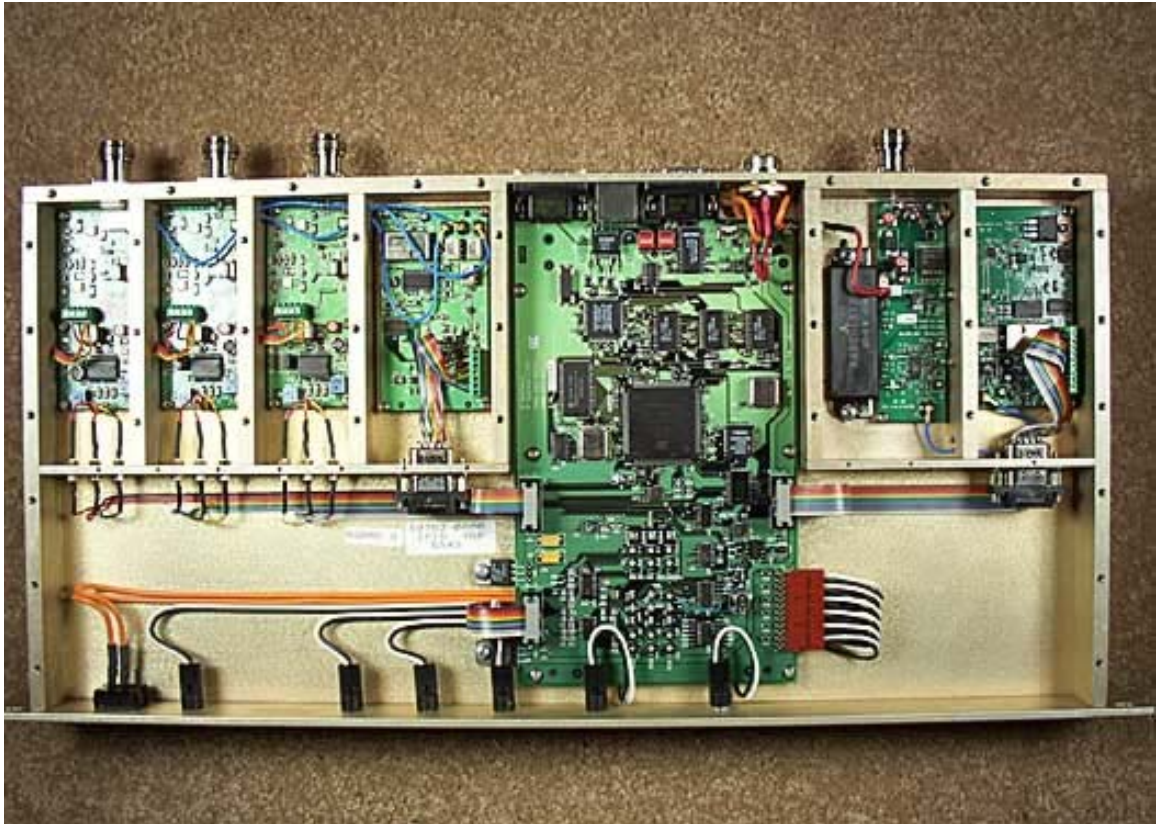
Internal Overall
