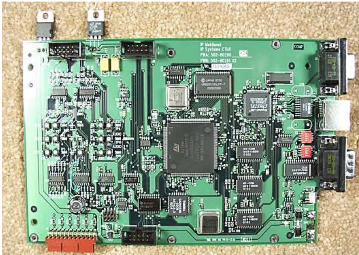
PCB 1 Top
