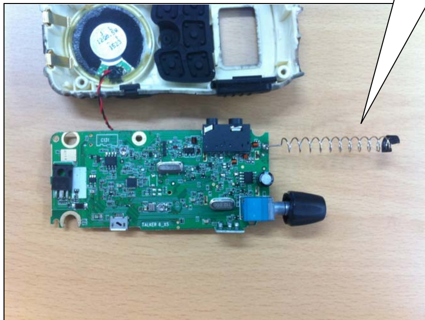
Helical Antenna
