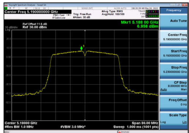
U-NII-1 Power spectral density-802.11 ax(40MHz),5190MHz,Ant0
