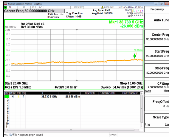
n77(3700-3980MHz) (20GHz-40GHz) 60M DFT-s-OFDM QPSK Inner 1RB Right High
