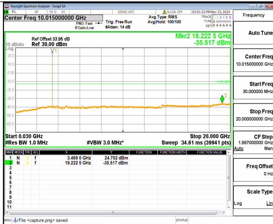
n78(3450-3550MHz) (30MHz-20GHz) 20M DFT-s-OFDM BPSK Inner_1RB_Right Low
