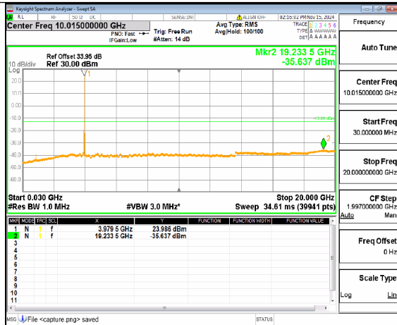
n77(3700-3980MHz) (30MHz-20GHz) 60M DFT-s-OFDM QPSK Inner 1RB Right High
