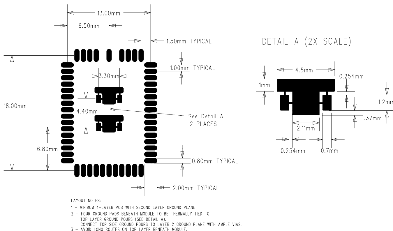
Figure 14 TiWi5 Recommended PCB Footprint (Top View)
