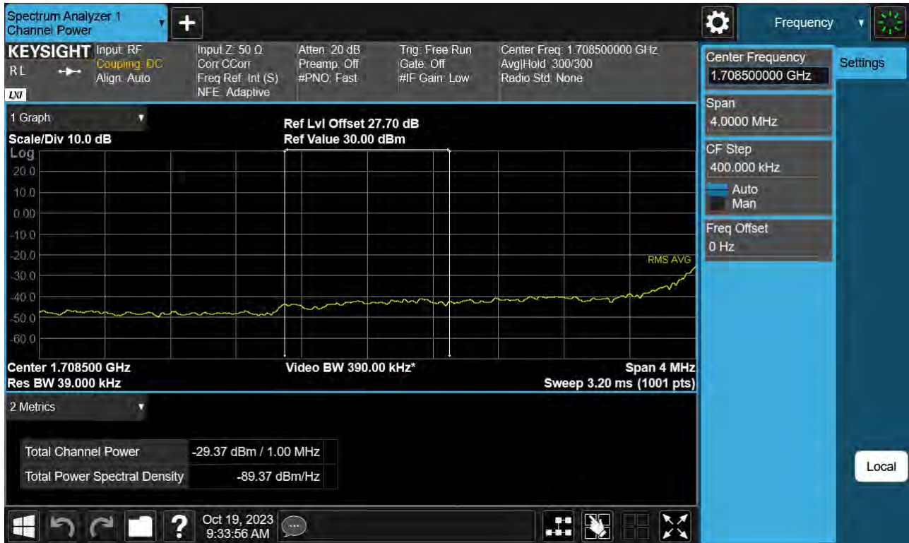
Sub6 n66. Lower Extended Band Edge Plot (35 M BW Ch.345500 BPSK_ Full RB) -3
