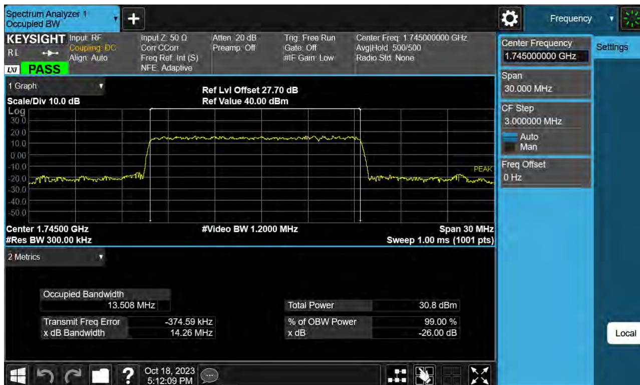
Sub6 n66. Occupied Bandwidth Plot (15 M BW Ch.349000 QPSK Full RB)
