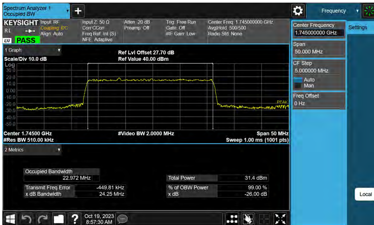
Sub6 n66. Occupied Bandwidth Plot (25 M BW Ch.349000 BPSK Full RB)
