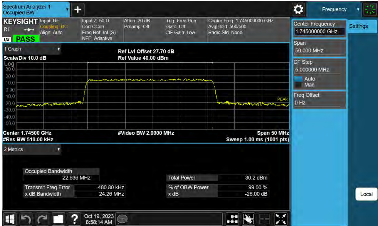
Sub6 n66. Occupied Bandwidth Plot (25 M BW Ch.349000 16QAM Full RB)
